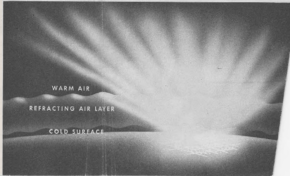
With a temperature inversion, light bends in refracting layer of air. A ray of light will thus be seen in areas far distant from its source.
