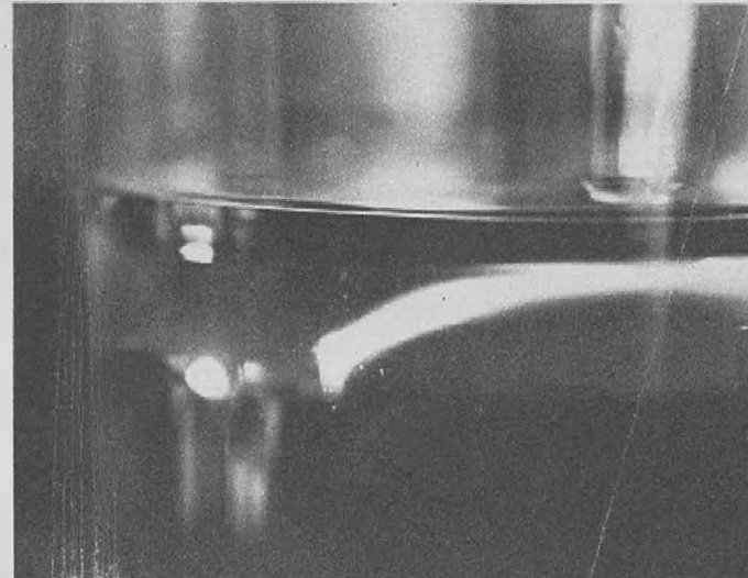
A light shining through the liquids bends at the meeting point. Same is true in air layers.
