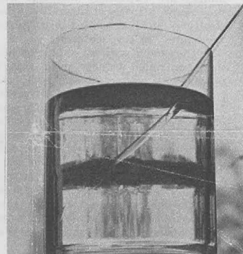
A glass rod seems to bend as it passes from one liquid to other. Light bends in this way.
