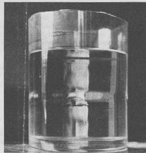
Acetone floating on benzene simulates air levels; lens effect distorts Dr. Menzel's face.
