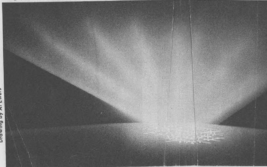
In normal air, light from the ground simply spreads out into space. Outside its range, where the earth curves away, there is darkness and no strange phenomena.
