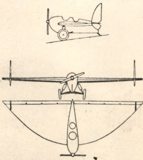
Fig. 15.—A 'parabola' aircraft by B. I. Tschernanowsky.
