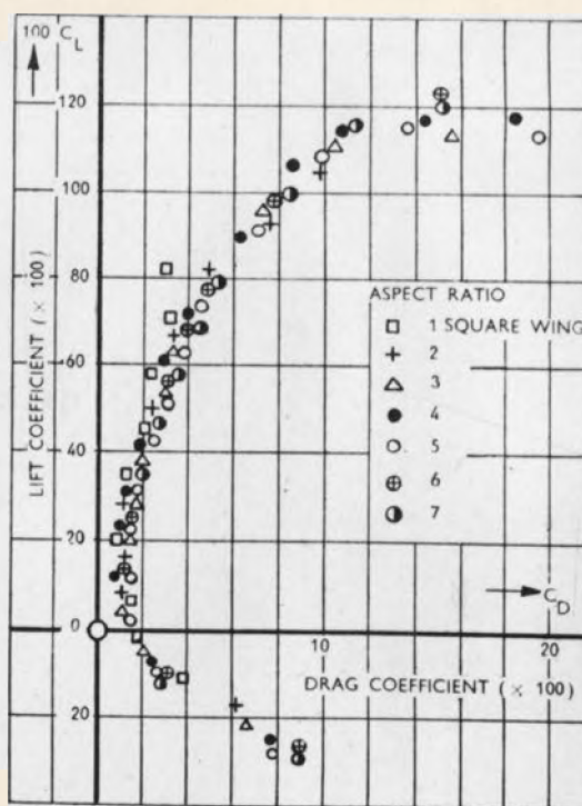
Fig. 20.—Lift and drag of wings of different aspect ratio. (Left) Wind-tunnel results obtained at Goettingen, in 1920; Goettingen 389 aerofoil with 10 per cent. thickness and square wing tips. (Right) A reduction of the results to an aspect ratio of five, by the Prandtl Aerofoil Theory of the induced drag, shows that a square aerofoil (aspect ratio of one) does not follow the theory. Its induced drag is less than predicted by the "horse-shoe vortex" assumption.
