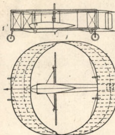
Fig. 6.—Huth annular biplane of 1909.
