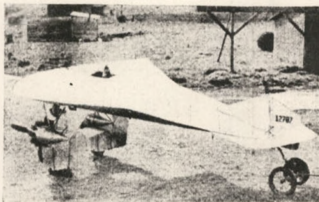
Fig. 19.—An American "Flying Flapjack" with two engines. It crashed while under test (1938).
