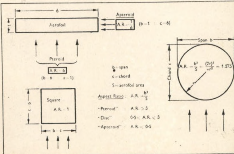
Fig. 2 (Right).—Definition of the aspect ratio of an aerofoil. The arrows signify the direction of the air flow against the wing. The terms pteroid (feather-like) and apteroid have been introduced by F. W. Lanchester.
