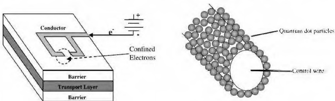
Figure 3. Programmable Materials. Various structures use electric fields to vary the confinement properties of quantum dots and can be assembled into bulk materials.
