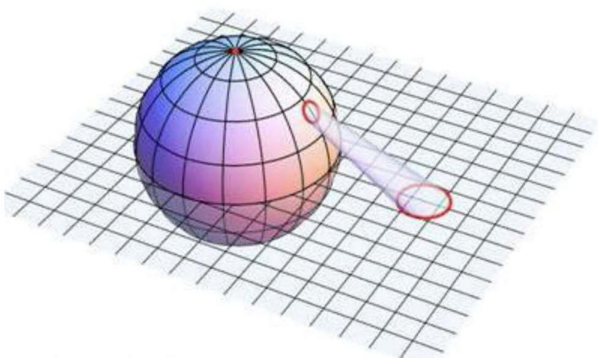
Figure 19. Stereographic Projection
