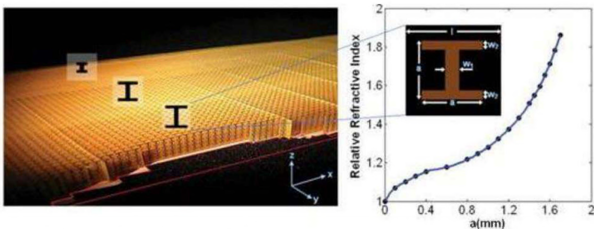
Figure 23. Implementation of the Ground-Plate Cloak 38
