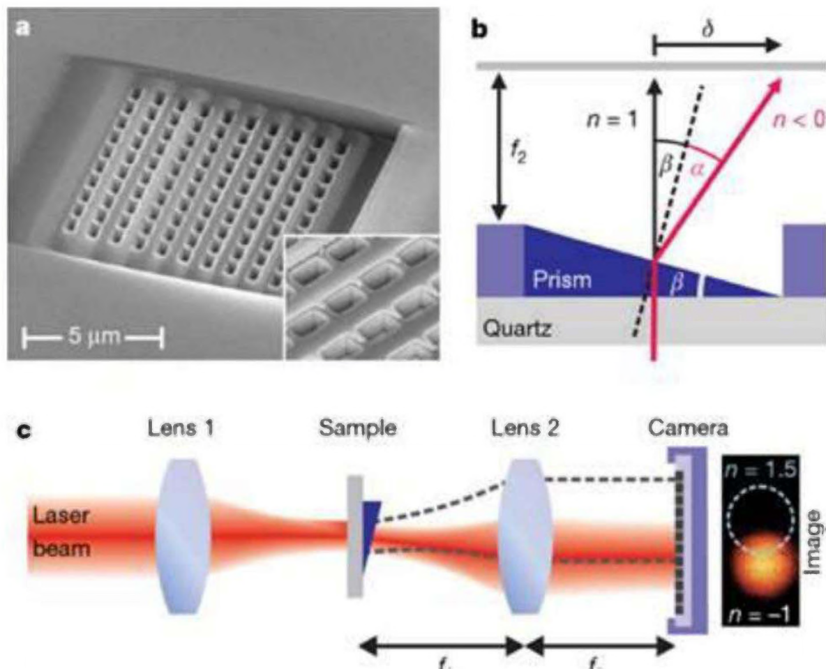
Figure 15. Demonstration of Negative Refraction With "Bulk" Optical Metamaterials Made of Nano-Fishnets 26
