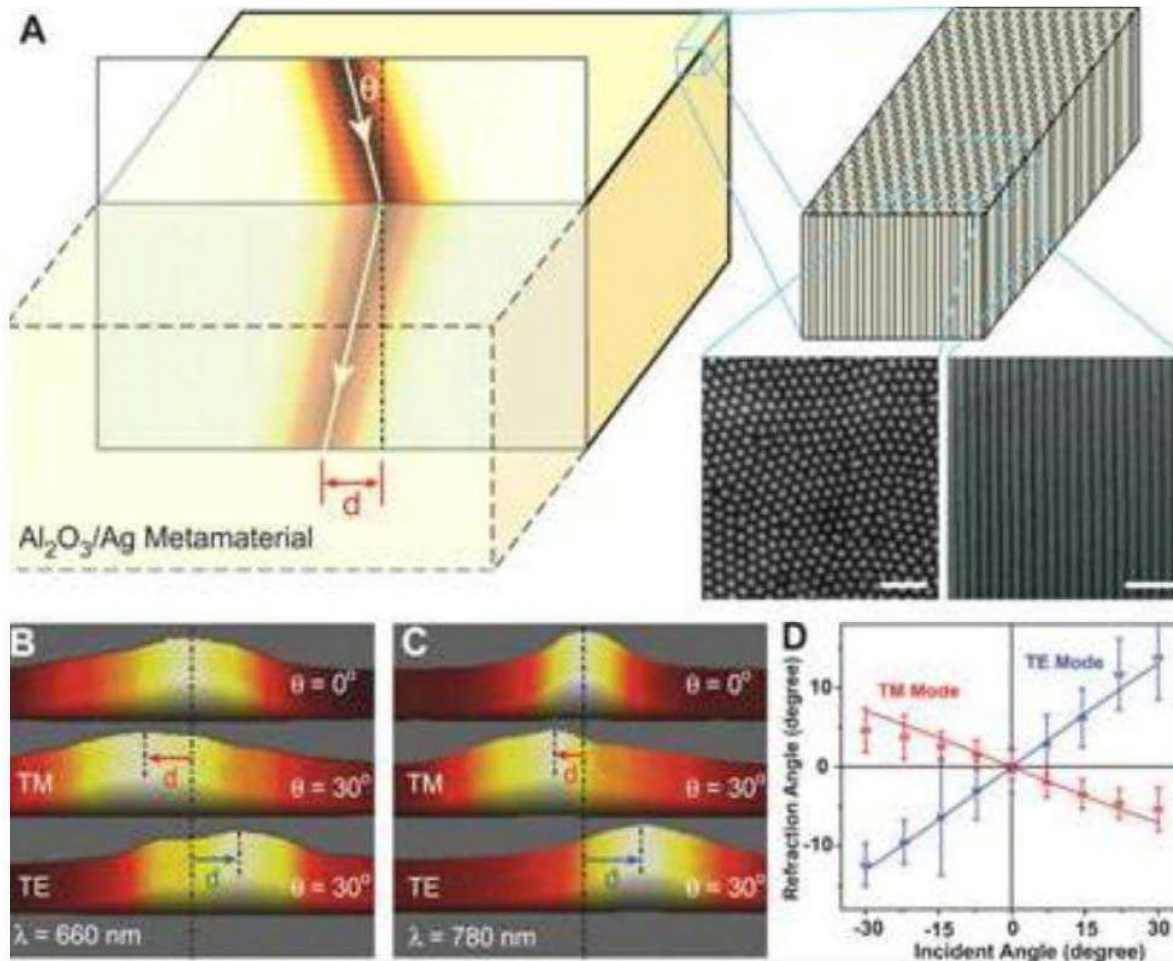
Figure 16. Demonstration of Negative Refraction With "Bulk" Optical Metamaterials Made of Nanowires 27
