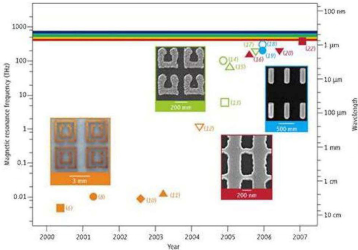
Figure 14. Advances in Metamaterials. The solid symbols denote materials with negative refraction; the open symbols denote optical materials with negative magnetic response. Orange: data from structures based on the double split-ring resonator (SRR); green: data from U-shaped SRRs; blue: data from pairs of metallic nanorods; red: data from the "fishnet" structure. The four insets give pictures of fabricated structures in different frequency regions. 22
