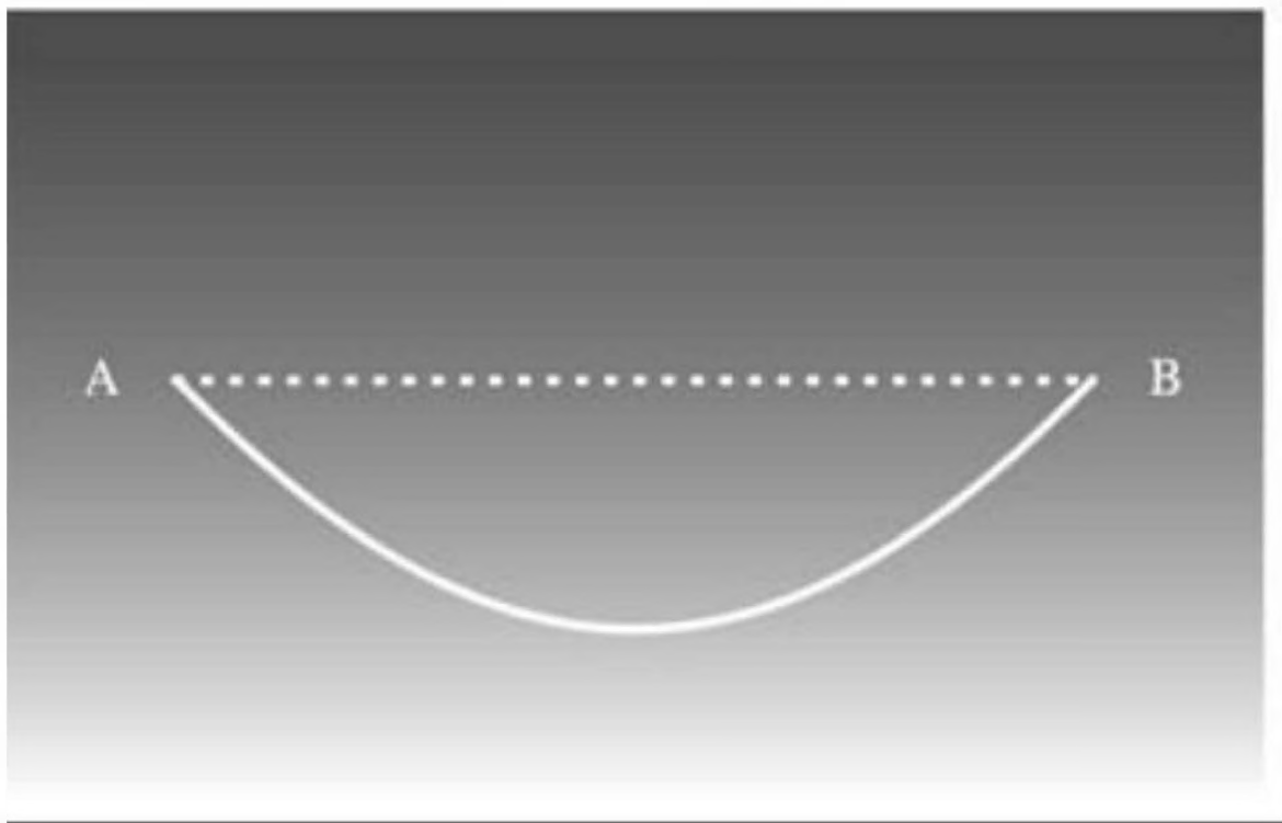
Figure 8. Fermat's Principle. The grey level indicates the refractive index. In traveling from A to B, light follows the path that takes the shortest time, traveling, if possible, through regions of low index.
