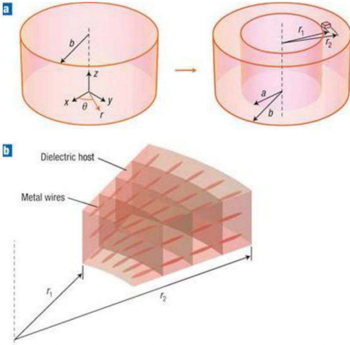
Figure 13. Idea for a Cloaking Device for Visible Light. Metal nanowires replace the split-ring resonators of the microwave cloaking device. Coordinate transformation and structure of the optical cloak. a: The coordinate transformation that compresses a cylindrical region r < b into a concentric cylindrical shell a < r < b . There is no variation along the vertical direction. The radii r_1 and r_2 define the internal and external radius of a fraction of the cylindrical cloak. b: A small fraction of the cylindrical cloak. The wires are all perpendicular to the cylinder's inner and outer interfaces, but their spatial positions do not have to be periodic and can be random. 20
