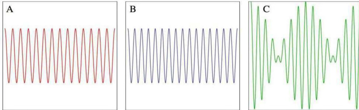
Figure 18. Wave Packets are Made by Combining Waves With Different Frequencies. The picture shows the simplest example: two waves (A and B) that add up to the wave packet (C).
