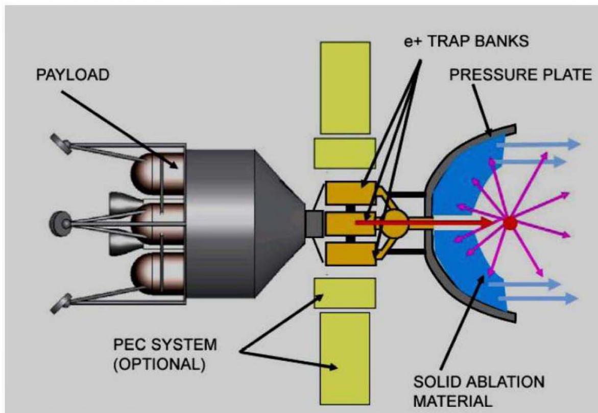
Figure 13. Modified Sänger Photon Rocket Concept (courtesy Positronics Research LLC) 39
