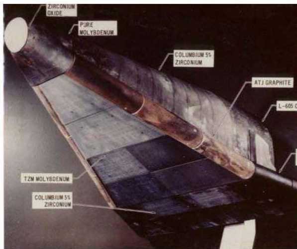
Figure 25. FDL ASSET Flight-Tested From Orbital Speeds To Evaluate 1960s' Materials. Carbon leading edges proved the least durable.
