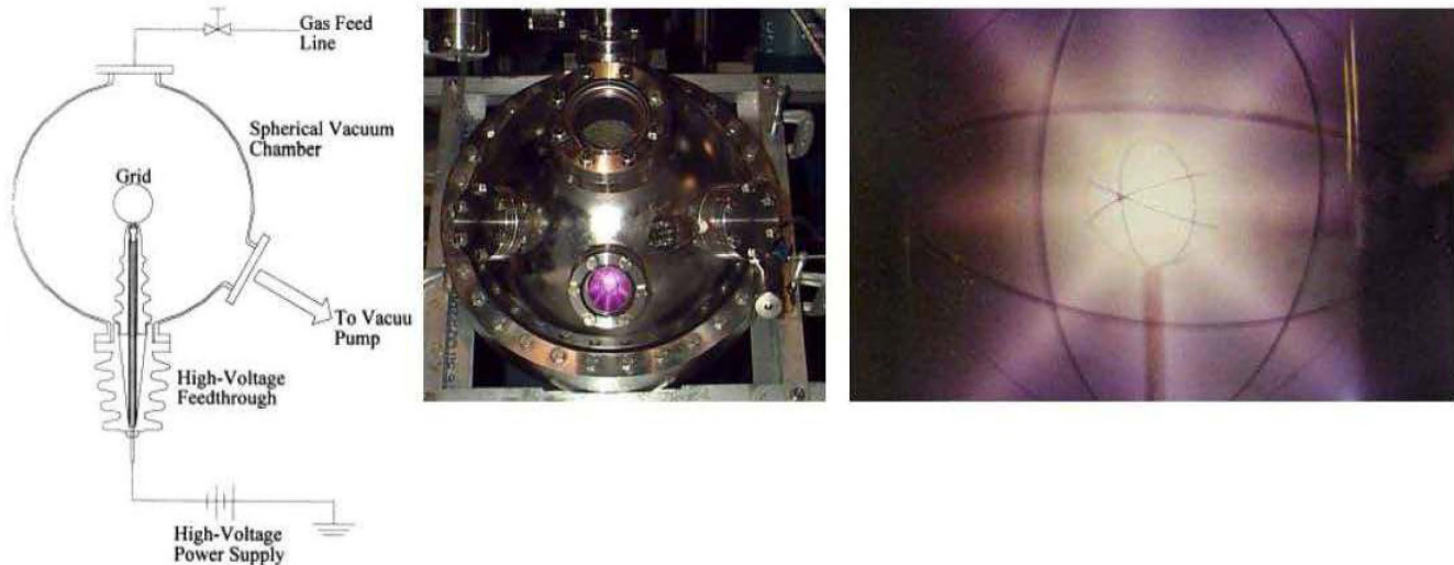
Figure 1.1. An UIUC Spherical IEC. The plasma discharge between the grid and vacuum wall creates an ion source that is extracted and directed towards the center by the highly charged negative grid. A photograph of a typical IEC chamber is shown in the center. A photograph of the discharge through the view port shows the "Star Mode" discharge where ion beams are created that pass through the grid openings. This is important for long run times since ion bombardment of the grids, hence grid wire sputtering, is minimized.
