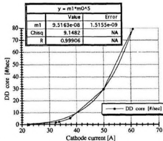
Figure 4.9. The D-D Fusion Reaction Rate Versus Cathode Current for dE_{\text{perp}, i} = 8\text{keV}
