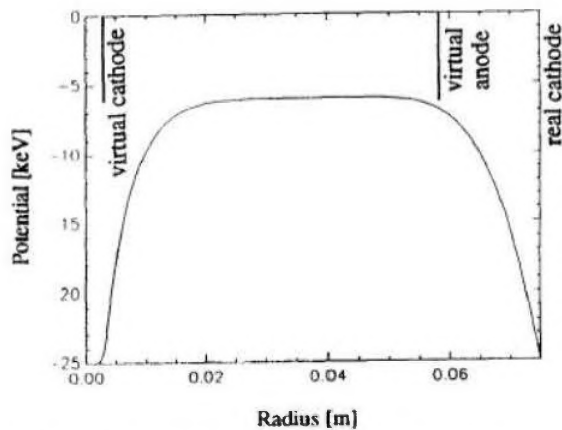
Figure 4.7. The Double Well Potential Calculated With IXL Code for d_{33\text{perp}} , i=14\text{keV} , I_i=55\text{A} , I_a=59\text{A}
