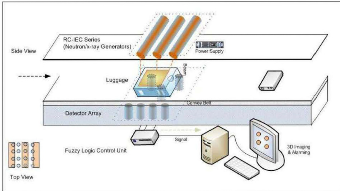
Figure 5.3. Further Illustration of the Integrated System for Airport Luggage Inspection. If desired, a second belt and detector array could be located above the IEC units to provide increased capacity.
