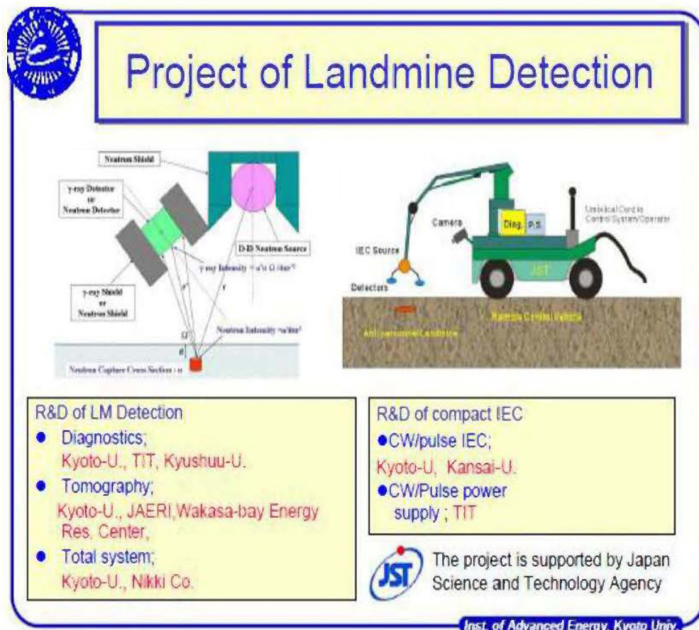
Figure 2.4. IEC Landmine Detection Project at Kyoto University
