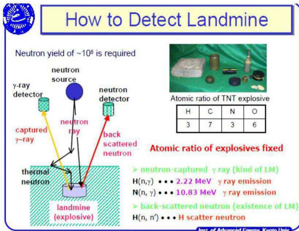
Figure 2.5. Scheme for Landmine Detection Using a Hybrid Magnetron Type IEC Neutron Source (From Reference 2.7)
