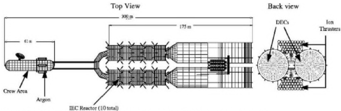
Figure 5.6. Scale Schematic of Fusion Ship II, a 750-MWe IEC Fusion Spacecraft
