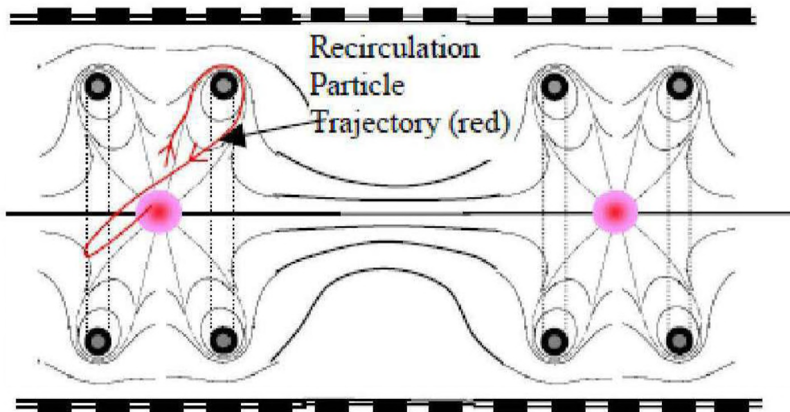
Figure 5.8. Diagram of Belt-Cusp Fields and Particle Recirculation
