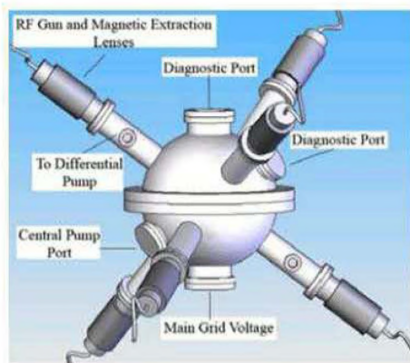
Figure 6.3. Multiple Ion Gun Concept
