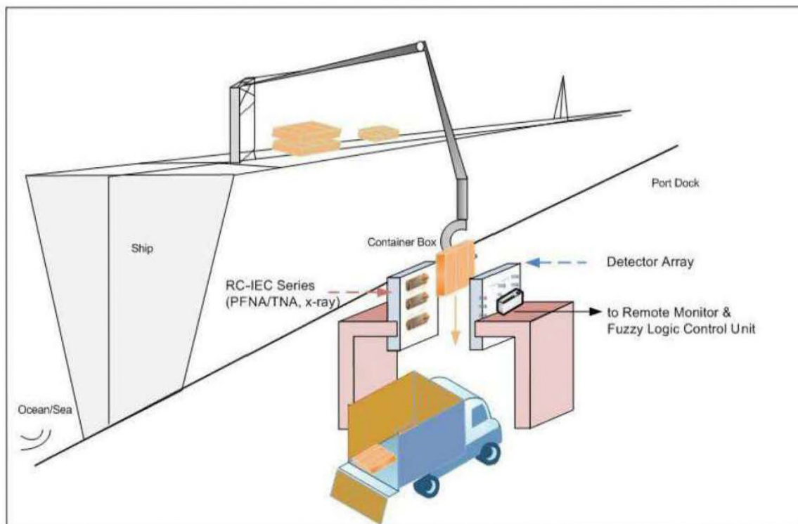
Figure 5.4. Further Illustration of the Integrated System for Ship Container Inspection
