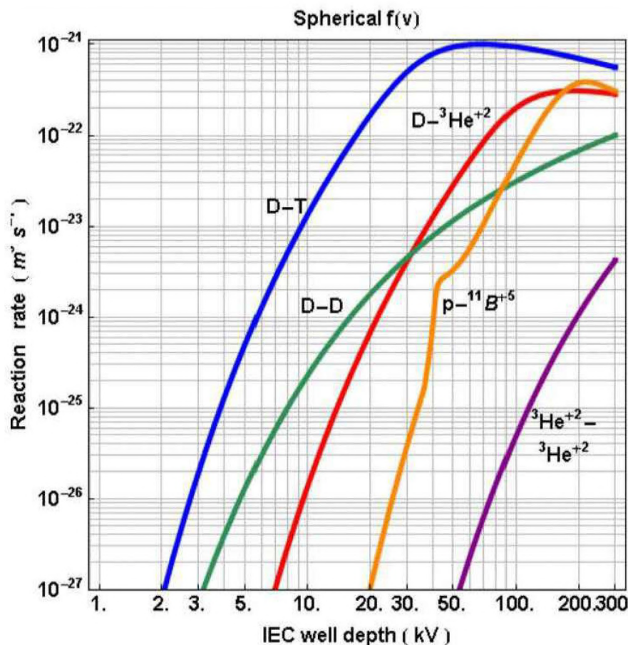
Figure 6.1. p- 11 B Fusion Cross Section Energy Requirements. The p- 11 B reaction rate approaches that of D-T at very high energies, i.e. deep potential wells.
