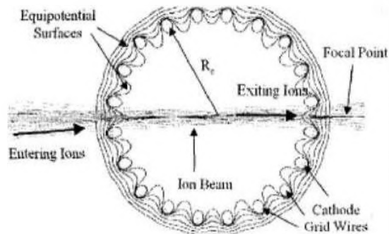
Figure 4.11. Diagram Showing Equipotential Surfaces of the IEC Cathode Grid and Their Focusing Effect on a Beam of Ions in the Star Mode Discharge at High Voltages (> 50 keV)
