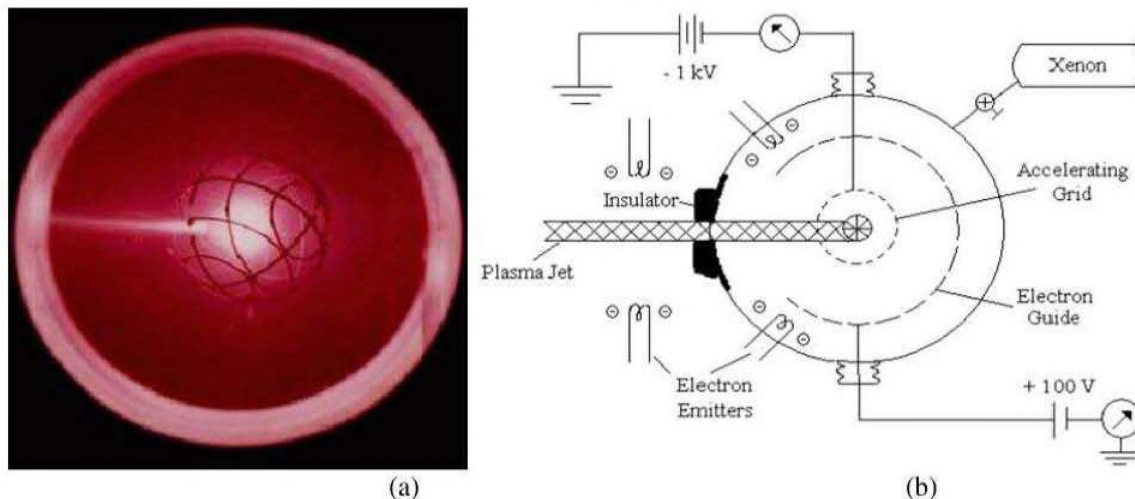
Figure 3.2. (a) Jet Operational Mode in Experimental IEC Device and (b) Jet Set-up
