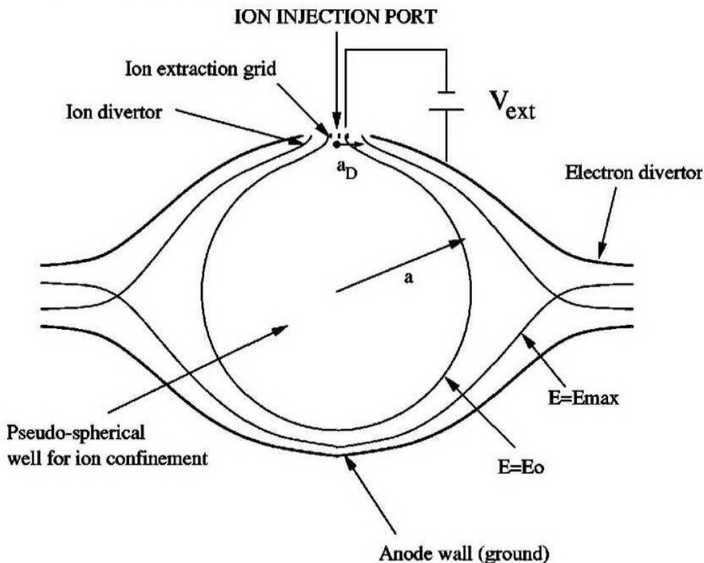
Figure 4.2. Detail of the Anode and the Ion Injection Port in PFX-I (not to scale). Ion and electron divertors are indicated, as well as the E_0 and E_{\max} equipotential lines that define the ion confinement region. The E_0 contour line determines the region of absolute ion confinement.
