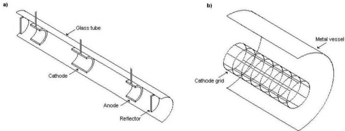
Figure 3.1. Two Types of Cylindrical IECs. The hollow cathode on the left (often termed the C-Device) and the 2-D gridded version on the right, often just called "the" cylindrical IEC.
