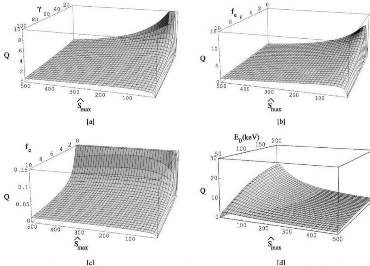
Figure 4.3. Plot of the Q-value (including electron losses) as a Function of (a) \hat{S}_{\max} and \gamma with f_e=10^{-3} , (b) \hat{S}_{\max} and f_e with \gamma = 5 , (c) \hat{S}_{\max} and f_e with \gamma = 100 , and (d) \hat{S}_{\max} and E_0 with \gamma = 5 and f_e = 10^{-3} . These plots have been obtained for E_0 = 100 keV [except (d)], \theta_0 = 0.01 , and \hat{E}_s = 1.04 . (Nomenclature is defined in Reference 4.2).
