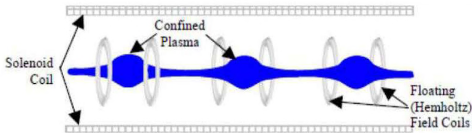
Figure 5.7. Illustration of a Three-Unit MCSA Device
