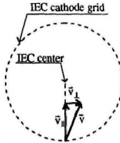
Figure 4.6. The Definition of the Parallel and Perpendicular Velocities at the IEC Cathode Grid
