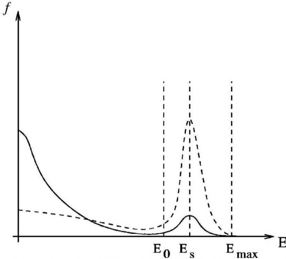
Figure 4.4. Sketch of Two Opposite Limits of the Beam-Maxwellian Equilibrium. The solid line corresponds to a case in which the Maxwellian population is dominant; the dashed line corresponds to a case in which the beam contribution is dominant.
