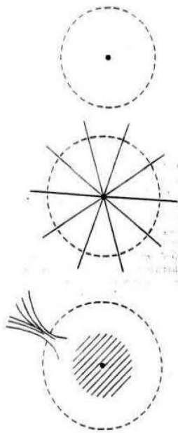
Figure 1.3. Discharge Modes in Gridded Devices Identified by Miley
