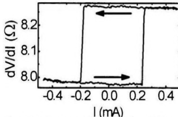
Figure 7. Spin-torque-driven magnetic switching for a Py20nm/Cu12nm/Py4.5nm spin valve with a 40 \times 120\text{-nm}^2 cross-sectional area, as the magnetization of the thin (free) magnetic layer is aligned parallel and antiparallel to the thicker magnetic layer by an applied current. (Reference 48)
