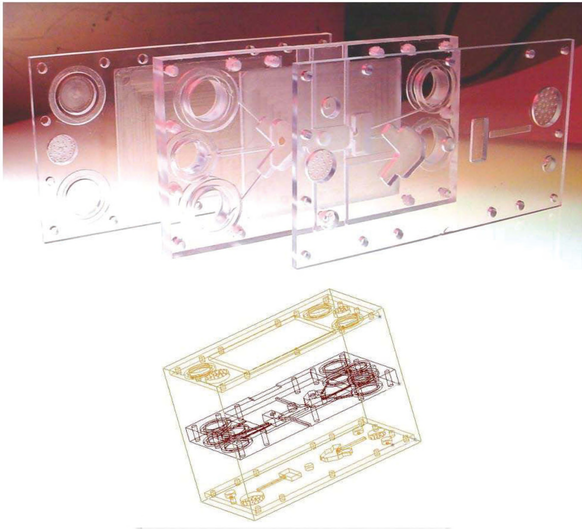
Figure 32. Design of an Automated Cell Culture System for NASA Space Applications Incorporating Microfluidics and Integrated Optical Components (Towe et. al.)
