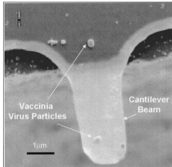
Figure 35. Scanning Electron Micrograph Showing a Cantilever Beam With a Single Vaccinia Virus Particle
