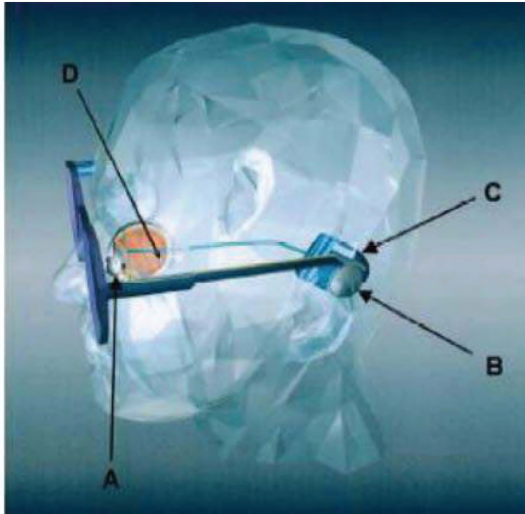
Figure 24. A Representation of the Retinal Prosthesis: (A) camera in the glass frame, (B) wireless transmitter, (C) extraocular electronic case (receiver), and (D) intraocular implant electrode array ( http://biomed.brown.edu/Courses/BI108/2006-108websites/group03retinalimplants/interocular.htm )
