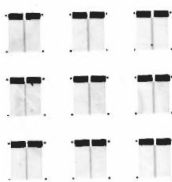
Figure 12. Photomicrograph 3 x 3 Array of Thermoelectric Glucose Sensors Constructed by Towe et al. at ASU
