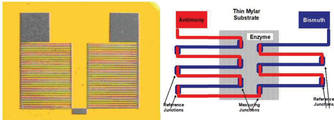
Figure 15. Thermopile Glucose Sensor (left) With Functional Illustration (right) are Made Using Photolithographic Techniques. This larger device is about 8 mm in length but has approximately 50 micron minimum geometries. (Towe et al.)
