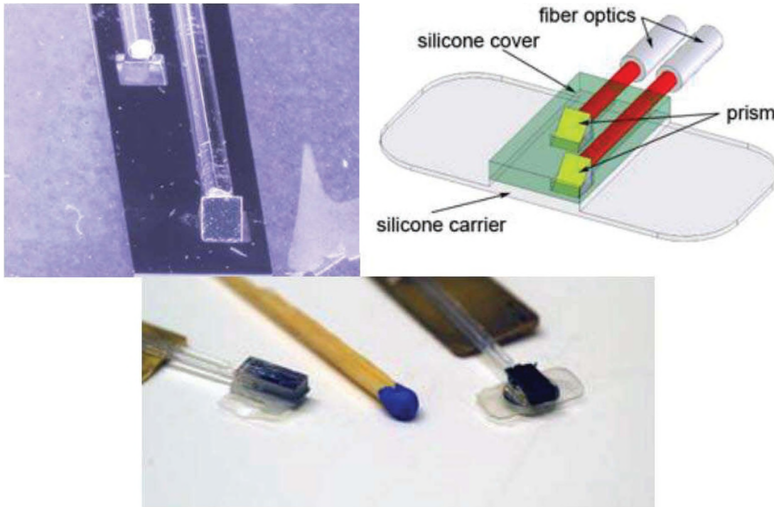
Figure 8. A Fiber Optical Oxygen Sensor Showing Two Optical Fibers Mated to Plastic Prisms That are Coated With an Oxygen-Sensor Coating, Usually a Fluorescent Ruthenium Compound ( http://www.imtek.de/content/projekte_en.php?ls=11 )
