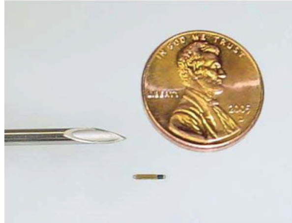
Figure 28. A New Generation of Implantable Neurostimulation Devices Can Pass Through the Lumen of a Syringe Needle. This device was made at ASU and is powered by ultrasound energy. (Towe et al.)
