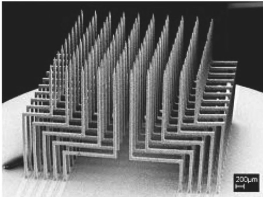
Figure 20. Scanning Electron Micrograph of a Brain Electrode Array Manufactured From Titanium and Produced by a Process of Electrodischarge Machining ("Electrical Discharge Machining and Chemical Etching", Fofonoff*, Martel, Hatsopoulos, Donoghue, Hunter)
