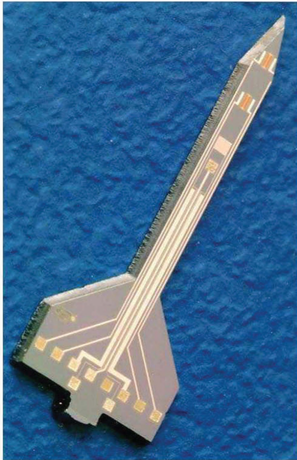
Figure 7. An ISFET (Ion Sensitive Field Effect Transistor) Needle-Type pH Sensor for Monitoring Tissue Physiologic Status ( http://www.ee.seikei.ac.jp/~selichi/lecture/Biomedical/09/09-biosensor.html )
