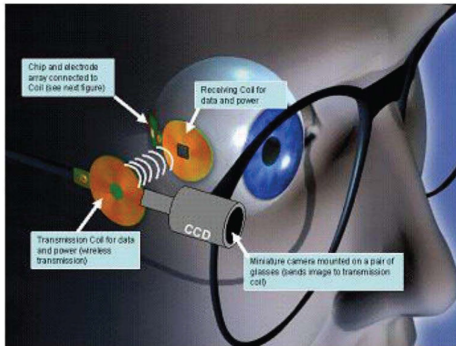
Figure 27. Power Transfer by Magnetic Induction to an Implanted BioMEMS Retinal Prosthesis. This is the Boston Retinal Implant Project.
