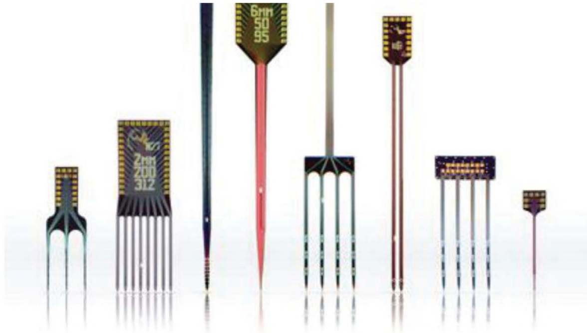
Figure 22. Polymer-Based Cortical Penetrating Neuroelectrodes Made by Processes of Thin Film Deposition and RF Etching (Neuronexus Inc)
