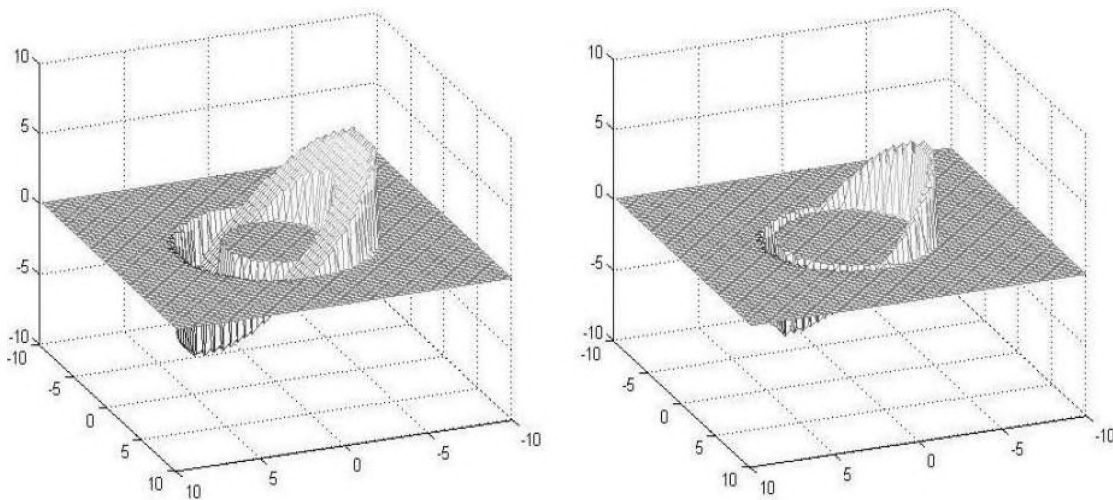
Figure 9. Two Images Illustrating the Contrast Between a Thick (left) and Thin (right) Shell Warp Bubble. A thin shell warp drive model has the capacity to dramatically reduce the energy requirements of a warp drive.
