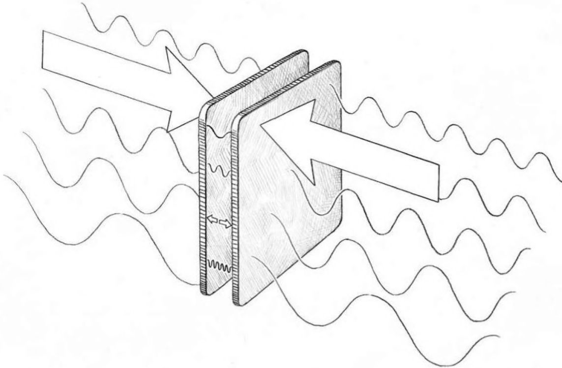
Figure 2. The Interior Region of Parallel Conducting Plates. The region experiences a reduced quantum vacuum energy density owing to the boundary condition the plates impose on the fields. This generates a measurable attractive force that pushes the plates together.
