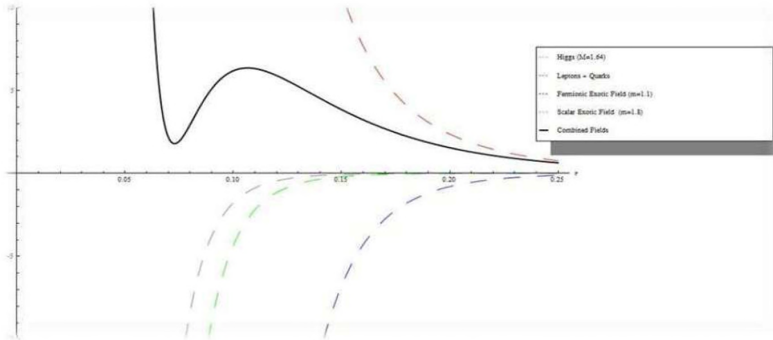
Figure 7. A Combination of Phenomenologically Viable Fields Generates a Stable Minimum of the Vacuum Energy Density at a Fixed Higher Dimensional Radius. This stable minimum, located at a positive energy, indicates a stable deSitter type spacetime and reflects a realistic dark energy model. Note in this plot that the radius of the extra dimensions is shown on the x-axis, and the energy density on the y-axis (normalized units are used).
