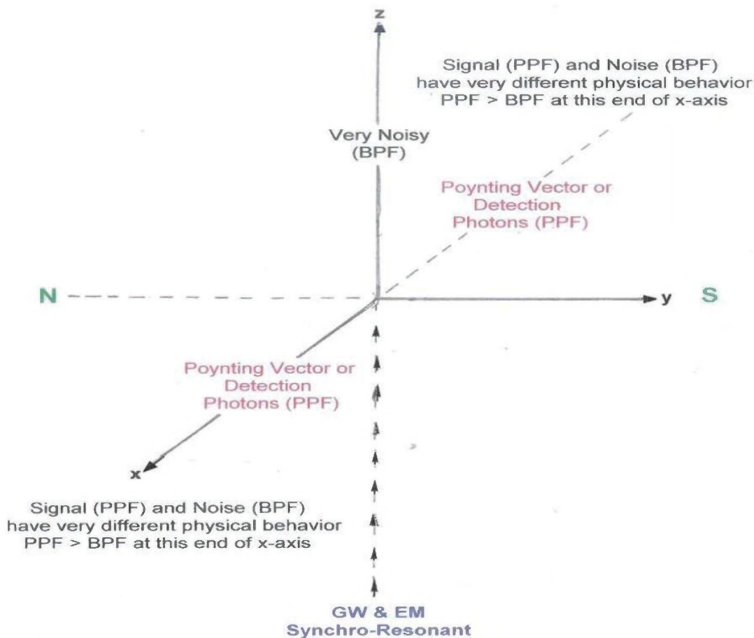
Figure 12. Detection Photons Sent to Locations That are Less Affected by Noise
