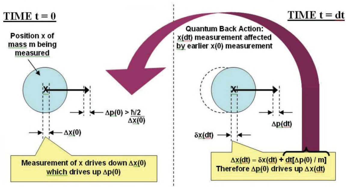
Figure 13. Quantum Back Action as a Mechanism for Creating the Standard Quantum Limit
