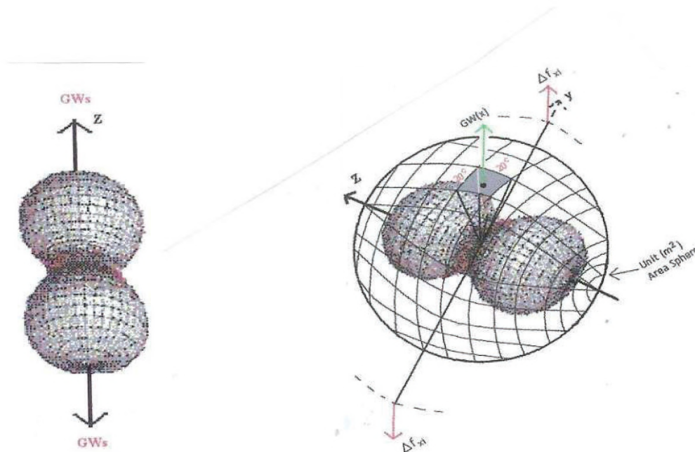
Figure 7. Omni-Directional Nature of the HFGW Radiation Pattern
