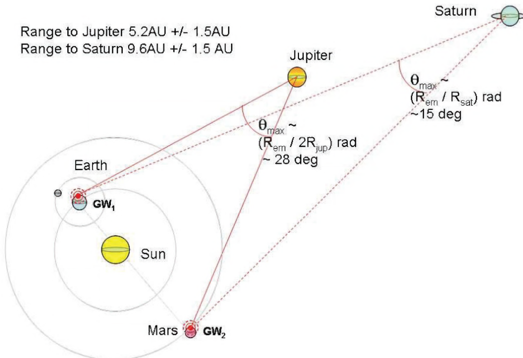
Figure 27. A GW Pair on Earth and on Mars for an Outer Planetary Reference Pair
