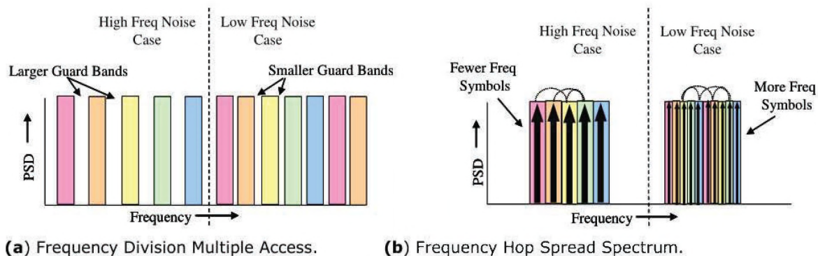
Figure 22. The Impact of Frequency Noise Improvements on FDMA and FHSS
