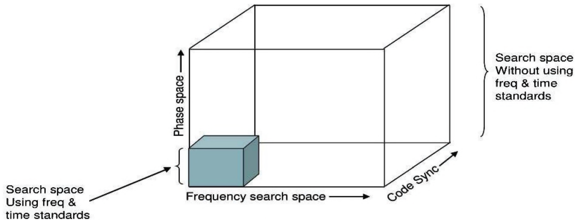
Figure 20. Acquisition Search Space Improvement Accruing from HFGW FTS
