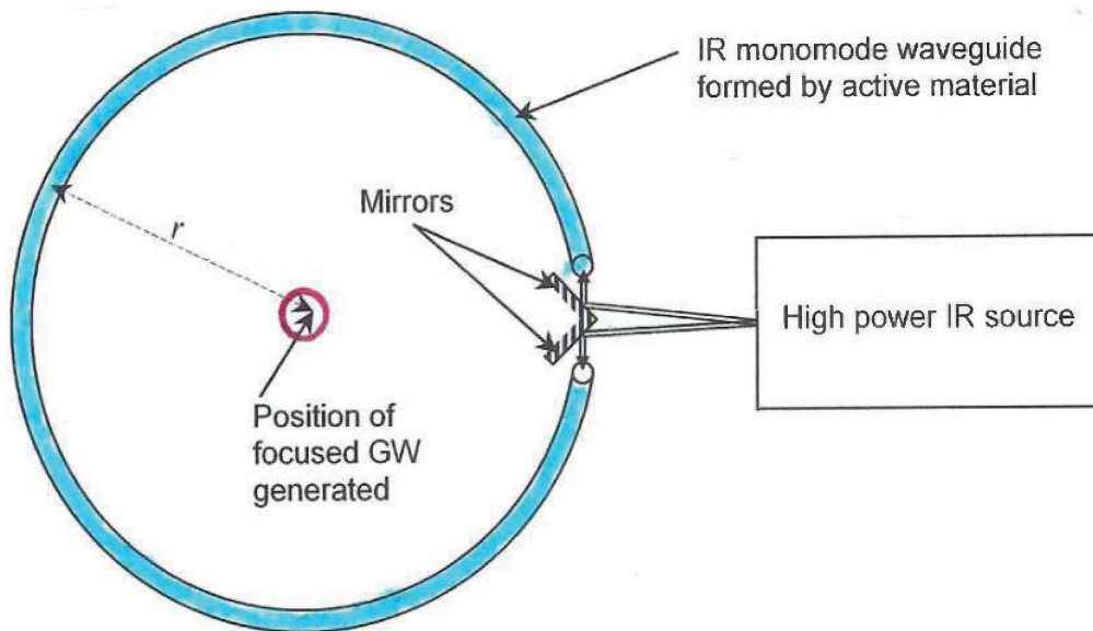
Figure 3. Circular Resonator Geometry Using Infrared Excitation
