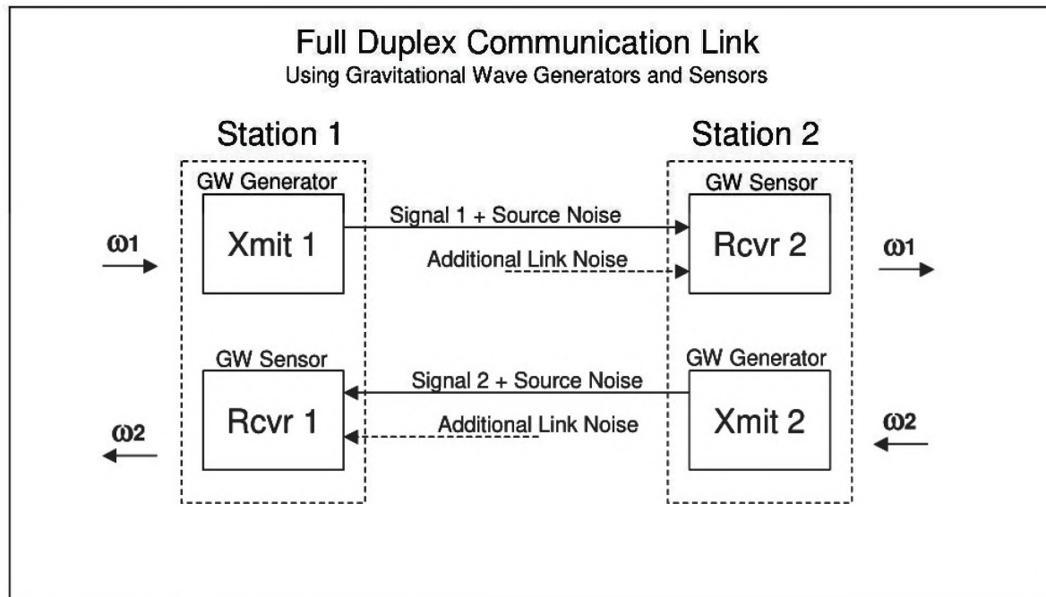
Figure 1. Communication Link Block Diagram
