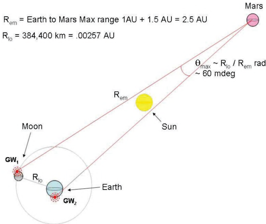
Figure 26. A GW Pair on Earth and on the Moon, as Used by a Mission to Mars
