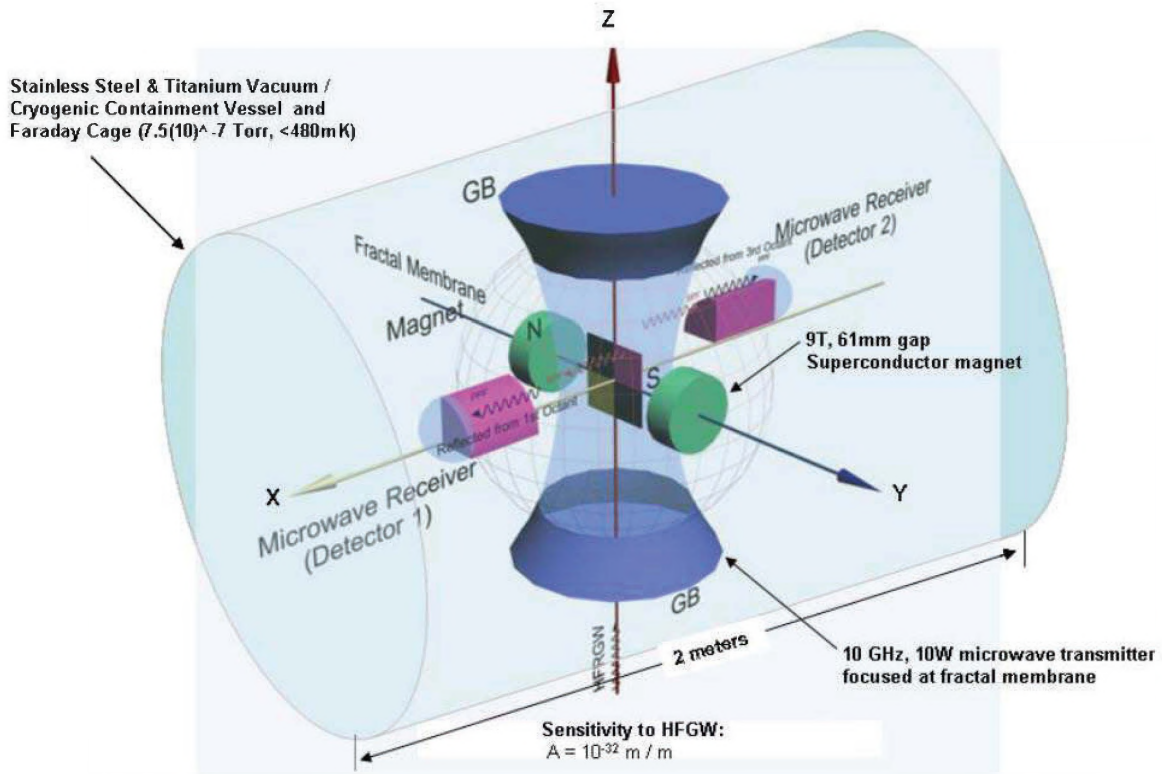
Figure 14. Schematic of Ultra-Sensitive HFGW Detector
