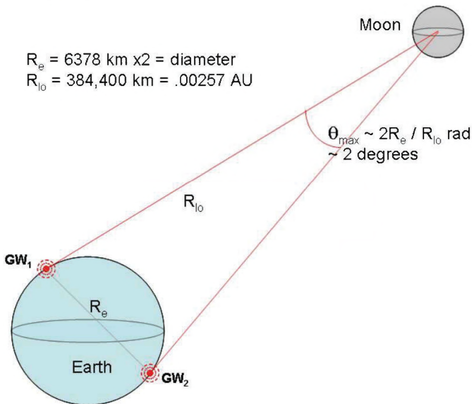
Figure 25. A GW Pair on Earth as Used by a Lunar Mission
