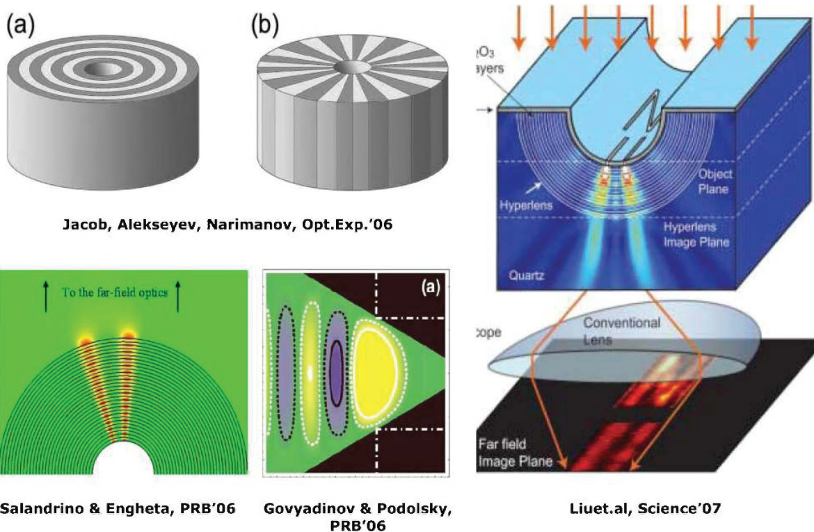
Figure 7. Theoretical Concepts (left panel) and Experimental Implementation (right panel) of an Optical Hyper-lens Capable of Magnifying Sub-Diffraction Objects to Observable (larger than \lambda/2 ) Size
