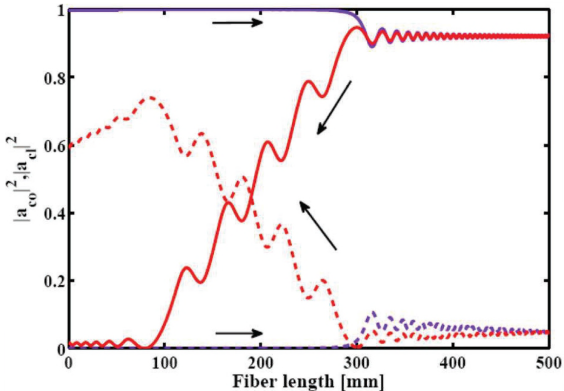
Figure 25. Example of Time-Irreversibility of Light Propagation Inside the Twisted Fiber Core: the core mode propagates with almost no loss from left to right (purple solid line), reflects back, and gets dissipated/mode converted on its way back (red line). Input mode is assumed to be right-hand circularly polarized (RCP). Mode conversion: into LCP cladding mode (dashed line). Propagation from left to right is represented by the red lines, from right to left: by the purple lines.
