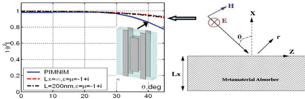
Figure 19. Wide-Angle Plasmonic Absorber Based on Negative Index Metamaterial. Right panel: schematic of an absorption-measuring experiment. A generic metamaterial with \epsilon_{yy} = \mu_{zz} = -1 + i , \mu_{xx} = 1 is assumed. Left panel: angular dependence of the absorption for a generic and specific (shown in the inset) metamaterial. Both exhibit wide-angle absorptivity. (Reference 20)
