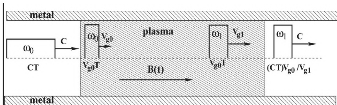
Figure 14. Schematic of Pulse Compression in Magnetized Plasma. A radiation pulse with initial frequency \omega_0 and duration T slows down in the plasma to a group velocity v_{g0} \ll c . Adiabatic spatially uniform variation of the magnetic field changes the radiation frequency to \omega_1 and increases the group velocity to v_{g1} \gg v_{g0} . The emerging pulse is compressed to T_1 = T v_{g0} / v_{g1} . (Reference 29)
