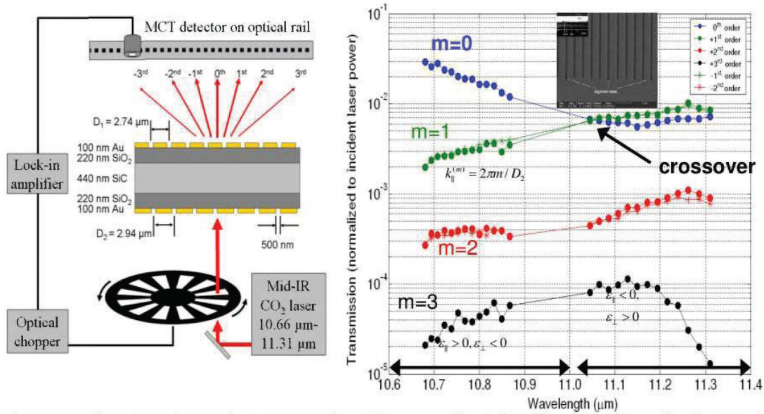
Figure 11. First Experimental Demonstration of Propagating Sub-Diffraction Waves in the IPM. (Left): Experimental setup demonstrating how sub-diffraction waves are launched into the IPM using FIB-fabricated sub-wavelength grating. Because the periods of the bottom ("launching") and top ("transforming") gratings are different, far-field observation of different harmonics of the bottom grating is enabled. (Right): Experimental results: the first sub-diffraction harmonic of the grating (green line) becomes stronger than the zeroth radiation-zone harmonic of the grating (blue line) in the region where \varepsilon_{\perp} > 0, \varepsilon_{\parallel} < 0 .
