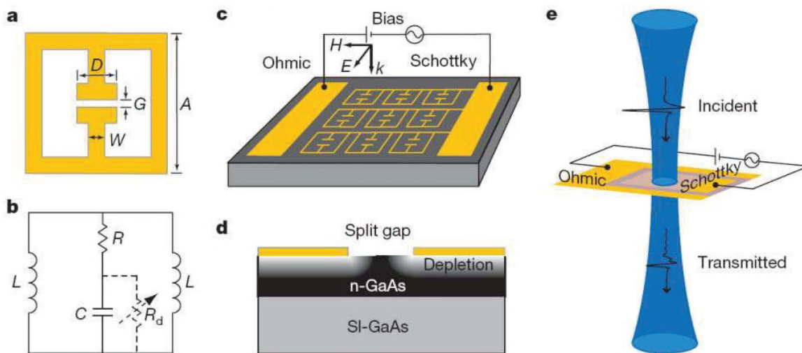
Figure 26. THz Properties of an Electric Split Ring Resonator. (a) Are controlled by applying voltage between Schottky and Ohmic contacts (c,d). (b) Schematic of circuit with inductance. Applied voltage controls charge density inside the split gap (d). The structure is investigated using a single-cycle THz pulse (e). (Reference 36)
