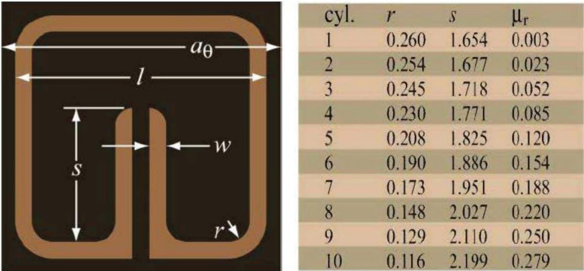
Figure 1. Example of a Metamaterial Component: The Magnetic Split Ring Resonator (MSRR) Design. The in-plane lattice parameters are a_y = a_z = 10/3 mm. The ring is square, with edge length l = 3 mm and tracewidth w = 0.2 mm. The substrate is 381 \mu\text{m} -thick Duroid 5870 ( \epsilon = 2.33 , t_d = 0.0012 at 10 GHz, where t_d is the loss tangent). The Cu film, from which the SRRs are patterned, is 17 \mu\text{m} thick. The parameters r and s are given in the table together with the associated value of \mu_r . (Reference 6)
