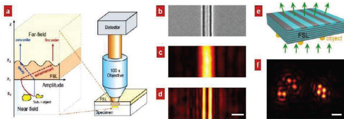
Figure 9. FSL Based on an Indefinite Permittivity Metamaterial Placed Between the Object and the Image-Releasing Grating. The grating releases into the far field sub-diffraction waves produced by light scattering off the object. The role of the metamaterial is to propagate sub-diffraction waves from object to grating. (Reference 27)
