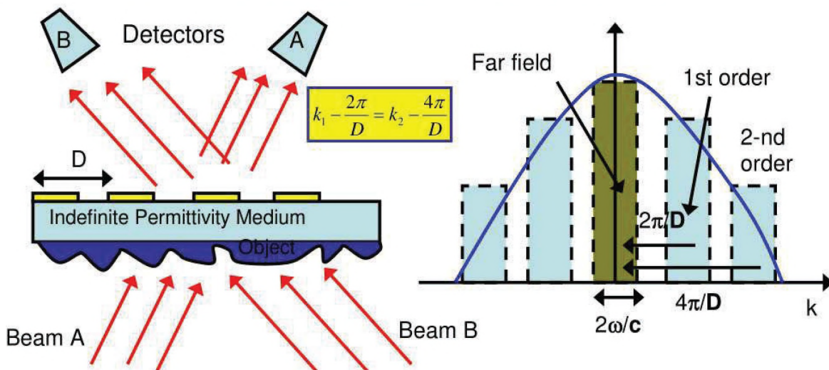
Figure 10. Tomographic Multi-Beam Multi-Detector Holography of Sub-Wavelength Objects Using Indefinite Permittivity Medium (IPM). Incident beam(s) scatter off the sub- \lambda object, propagate through the IPM, and then get re-scattered into the far field by the grating with the period D . The purpose of the multi-detector arrangement is to disentangle the k_1 and k_2 spatial wave numbers in the object's spectrum (shown in the left panel). Beams A and B are phase-shifted with respect to each other.
