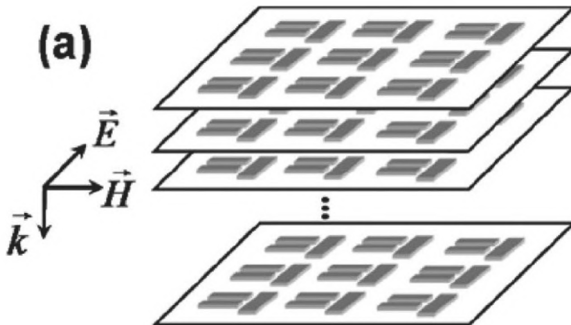
Figure 17. True Multi-Layer Metamaterial With a Unit Cell Shown in Figure 15: radiative antenna (single metal strip) coupled to a dark antenna (two perpendicular metal bars). Such metamaterial exhibits “slow” light propagation along the incidence direction (slowed down by a factor 30 or more). (Reference 32)
