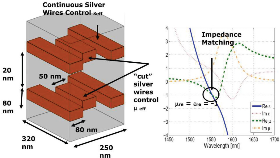
Figure 20. Specific Design of a Wide-Angle Plasmonic Absorber Based on Negative Index Metamaterial Operating at \lambda=1550 nm. Left panel: Schematic of the silver-based plasmonic structure. Right panel: Extracted permittivity and permeability for the normal incidence demonstrate impedance matching: \epsilon_{yy} = \mu_{zz} = -1 + i . (Reference 20)
