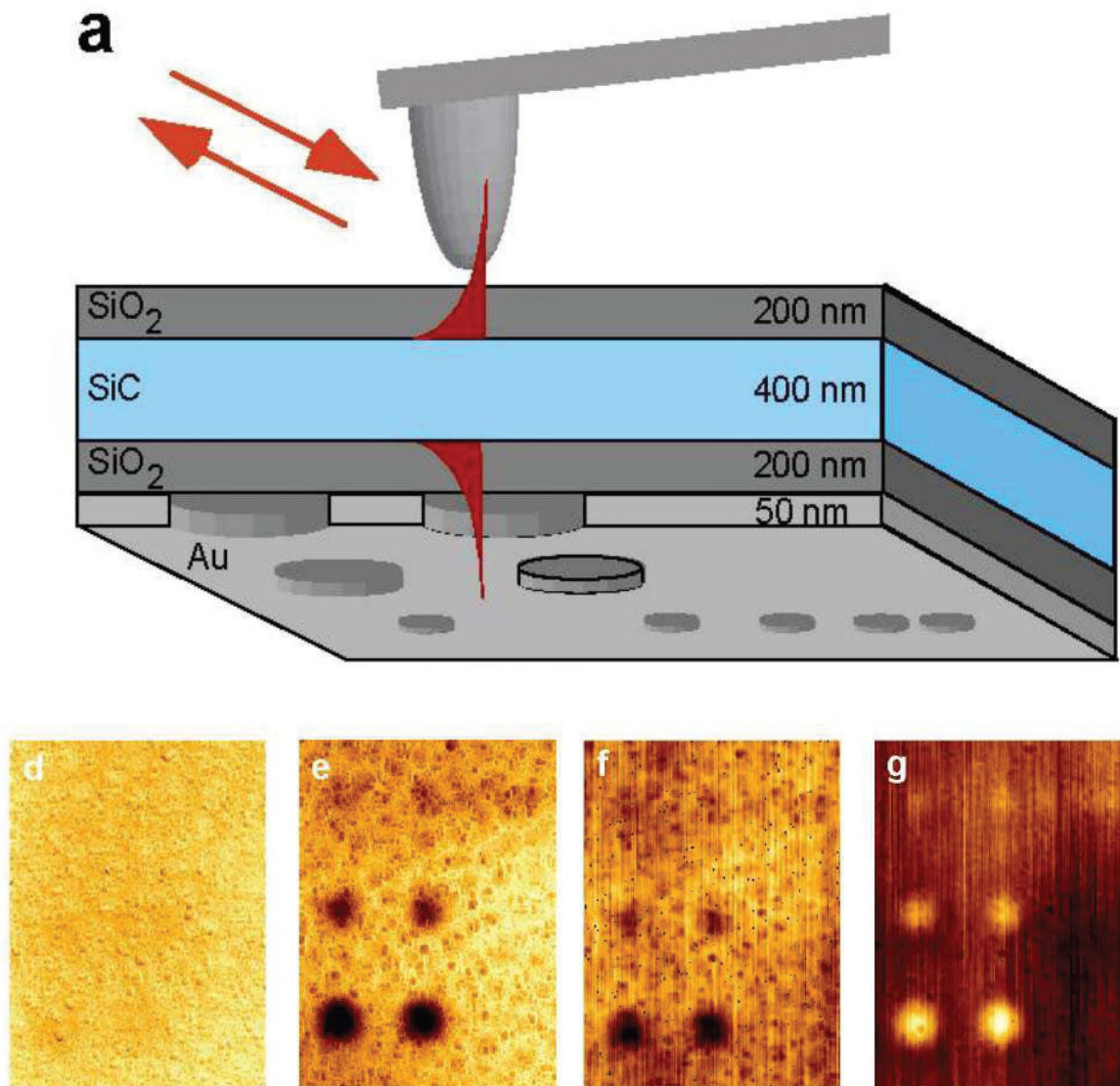
Figure 6. Schematic of the SiC-Based Super-Lens Which is Imaging Sub-Wavelength Holes Buried Under the SiO 2 Layer. The imaged objects are \lambda/20 holes milled in gold using FIB. The scattered signal is picked up by the tip of an NSOM and directed towards the IR detector. Depending on the imaging wavelength, either amplitude (e) or the phase (f,g) of the signal are prominent.
