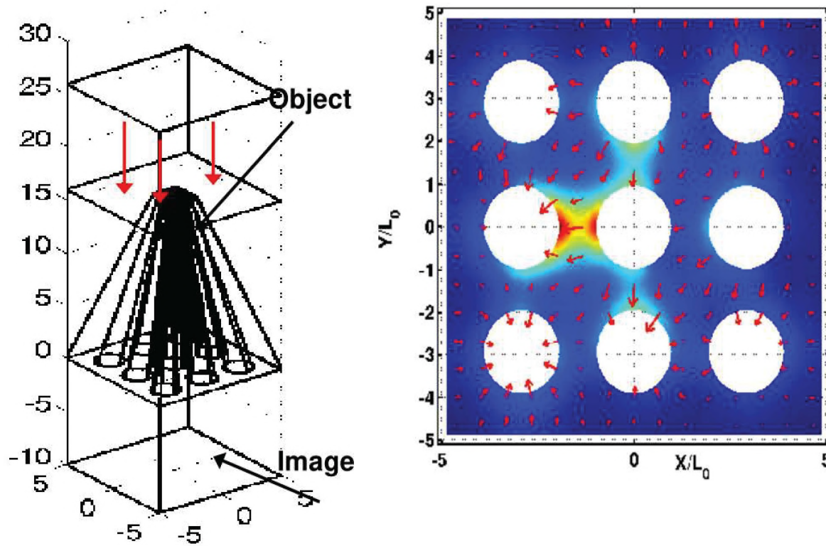
Figure 8. Hyper-Lens Based on a Converging Array of Metal Wires. A small object can be placed at the tip, illuminated from the top, and magnified by the expanding array of wires. Left panel: schematic. Right panel: \lambda/25 object magnified by a factor 5x by the expanding hyper-lens. This hyper-lens can operate at mid-IR frequencies. (Reference 26)
