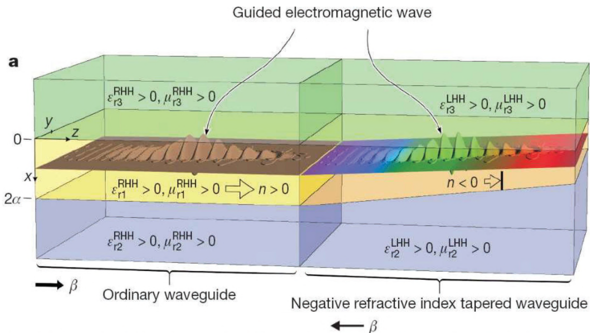
Figure 15. Trapped Rainbow: A Waveguide with Negative Index Core Can Stop Light. A guided wave packet is efficiently injected from the ordinary waveguide to the left-handed heterostructure LHH (see also Figure 4), inside which it propagates smoothly owing to the slow (adiabatic) reduction in the thickness of the core. The smallest (red) frequency components of the wave are stopped at the smallest core thicknesses of the LHH, while the largest (blue) components stop at correspondingly larger core thicknesses. (Reference 30)
