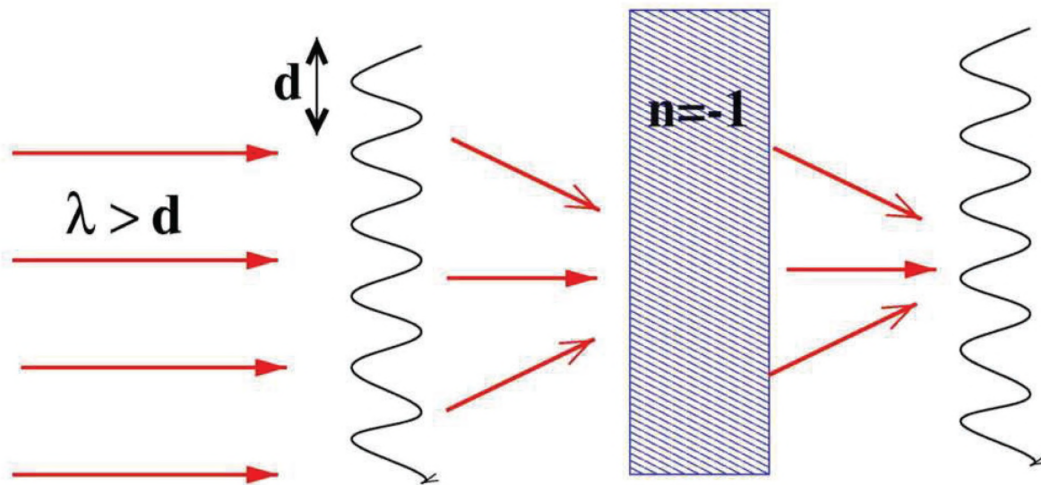
Figure 5. Schematic of the Super-Lens with n=-1 Refractive Index Corresponding to (\epsilon = -1, \mu = -1) Surrounded By Vacuum. Super-lens' presence enables imaging sub-diffraction objects such as the periodic grating shown here.
