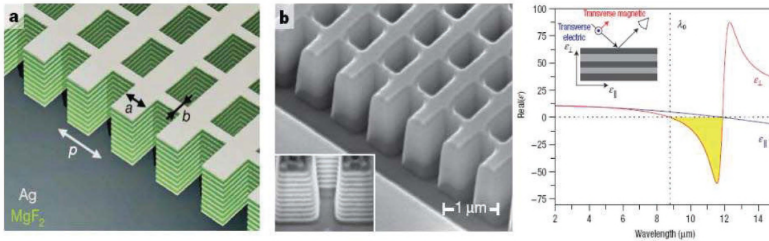
Figure 4. Recent Optical Metamaterials for Telecommunication Wavelength \lambda = 1.5 \mu\text{m} (Left and Middle) and Mid-Infrared IPM. The multi-layer fishnet is made of silver films separated by a dielectric spacer. A focused ion beam was used to produce the prism-shaped fishnet. The IPM was obtained by depositing interleaved 80 nm layers of \text{In}_{0.53}\text{Ga}_{0.47}\text{As} and \text{Al}_{0.48}\text{In}_{0.52}\text{As} . The layers, approximately 8.1 \mu\text{m} thick, grown by molecular beam epitaxy on lattice-matched InP substrates. The InGaAs layers were uniformly doped to create different values of permittivity in alternating layers. (Reference 10 and 11)
