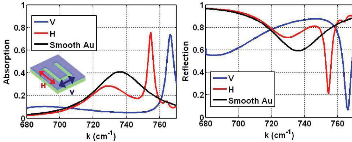
Figure 22. Preliminary Attempts to Design a Better Absorber Using Complementary MetaMaterials (U-shaped CMM). Note that only 40 percent absorptivity is possible with a smooth gold film. Paradoxically, this absorptivity increases to 75 percent when the metal mirror is made "leaky" by perforating it with an array of CMMs (left panel).
