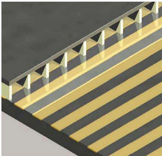
Figure 7. Alternative Apparatus for Ground State Energy Suppression: Casimir Strip and Spacer-Channels
