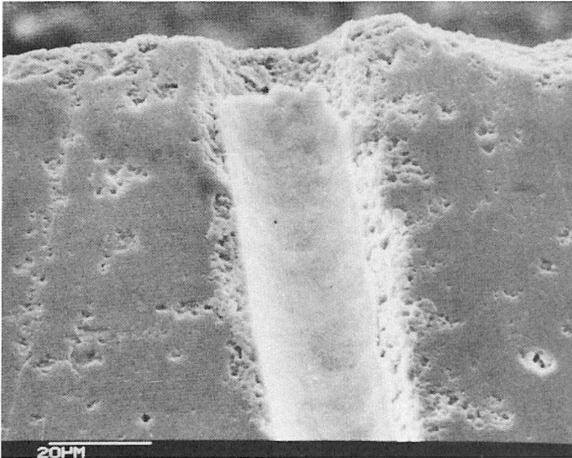
Figure 12. SEM of EV Damage to Ceramic Plate (20 um scale) (Reference 36)
