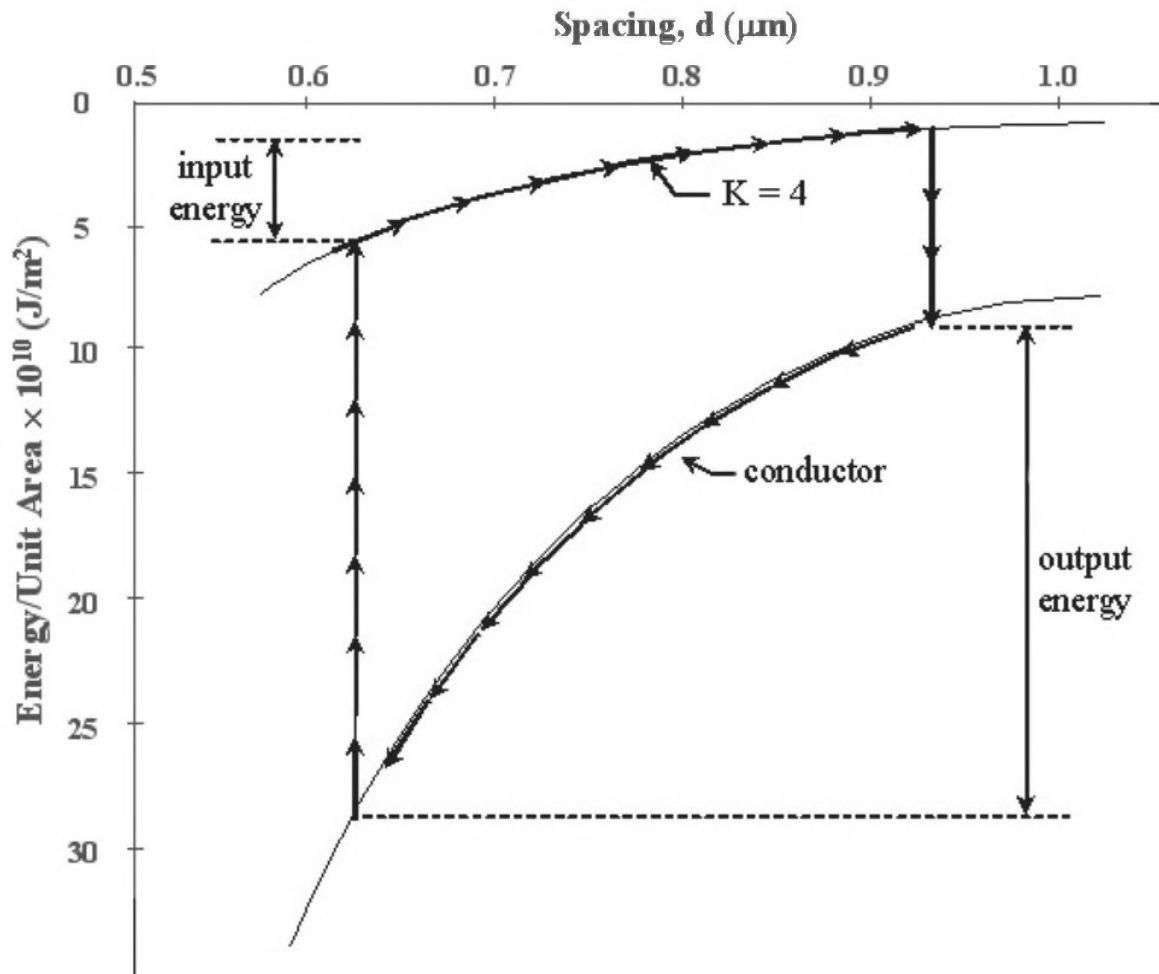
Figure 10. Tunable Casimir Effect: Engine Cycle
