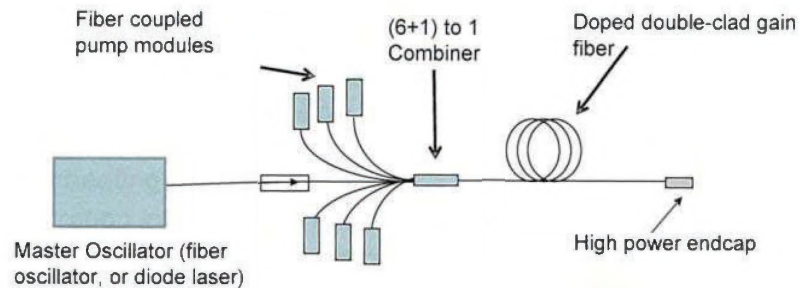
Figure 22. Typical HPFL MOPA Design (courtesy of the Directed Energy Professional Society).
