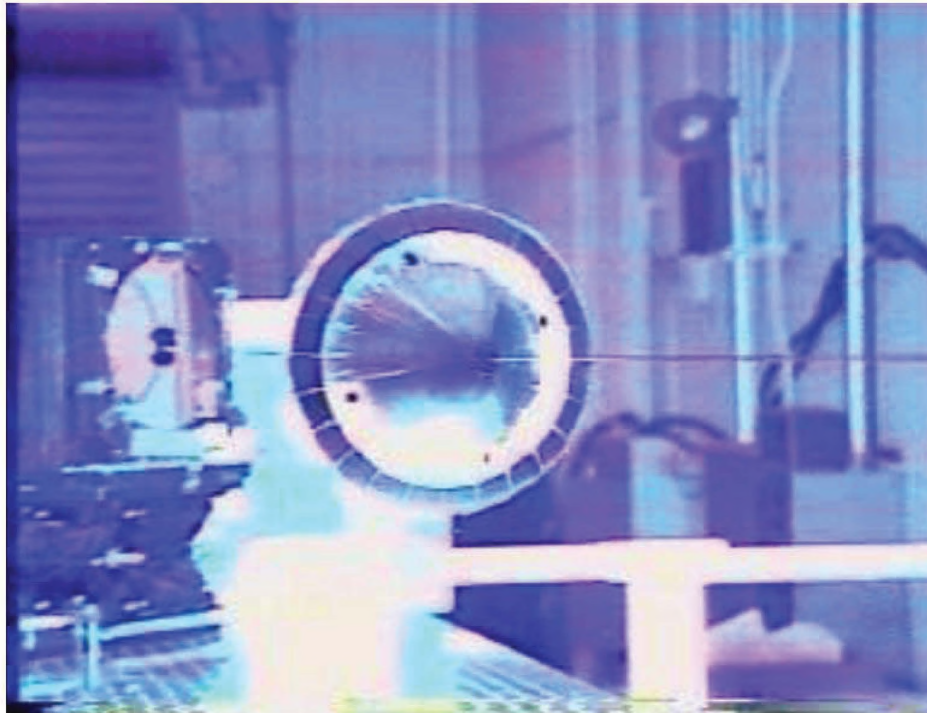
Figure 6. Lightcraft Undergoing Horizontal Guide-Wire Flight Test (courtesy of F. Mead, AFRL/PRSP, Edwards AFB, CA).
