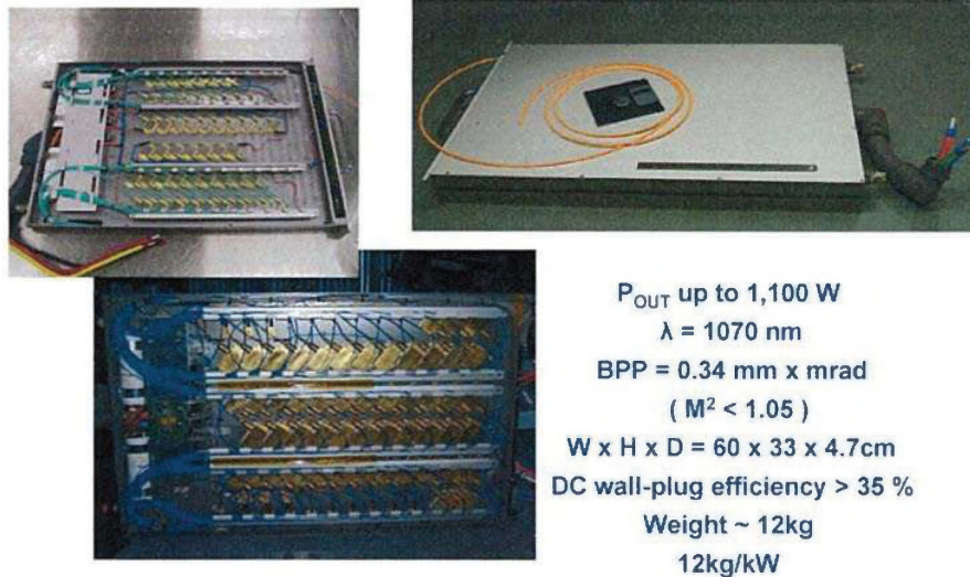
Figure 26. Single Mode Fiber Laser Modules (courtesy of IPG Photonics).
