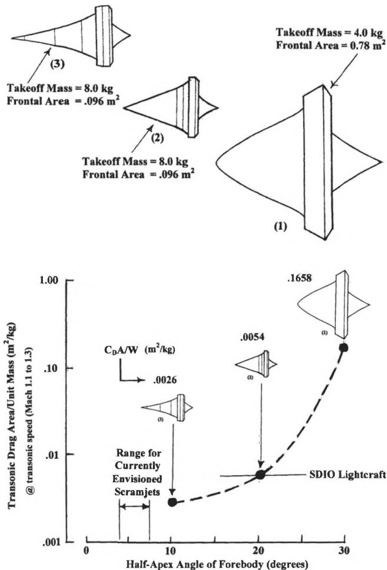
Figure 9. Lightcraft Vehicle Evolution (in 3 steps) [26].
