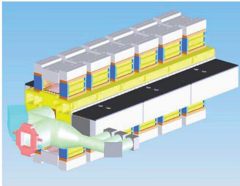
Figure 20. DARPA's High Energy Liquid Laser Area Defense System (courtesy of P. Saunders, AFRL/RDS, Kirtland AFB, NM).
