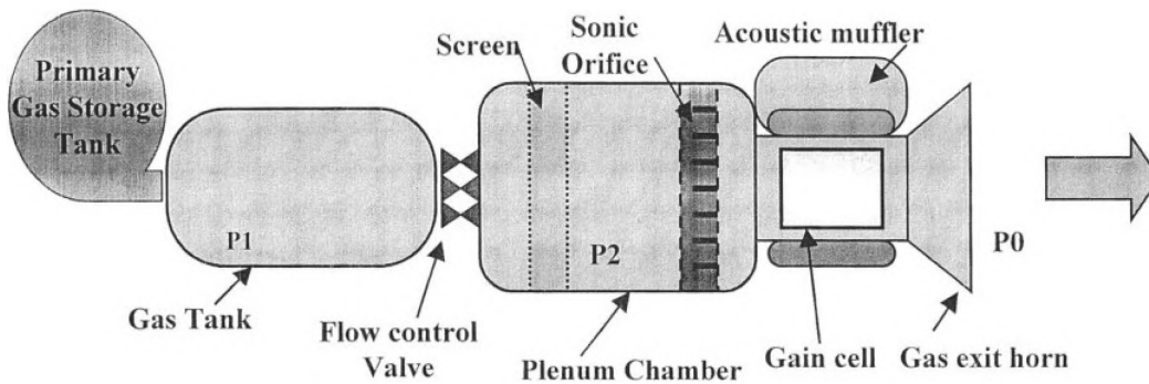
Figure 17. Schematic of MOPA [29].
