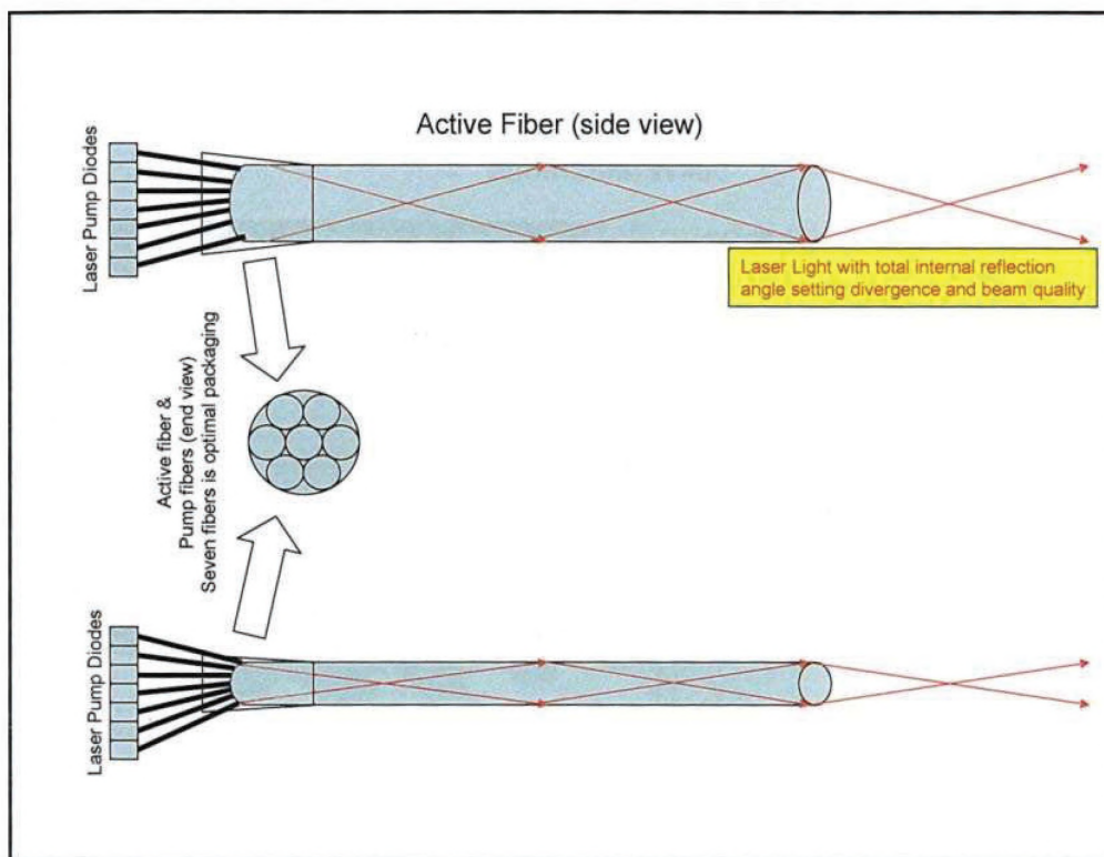
Figure 25. Large and Small Diameter Fiber Lasers (courtesy of the Directed Energy Professional Society).
