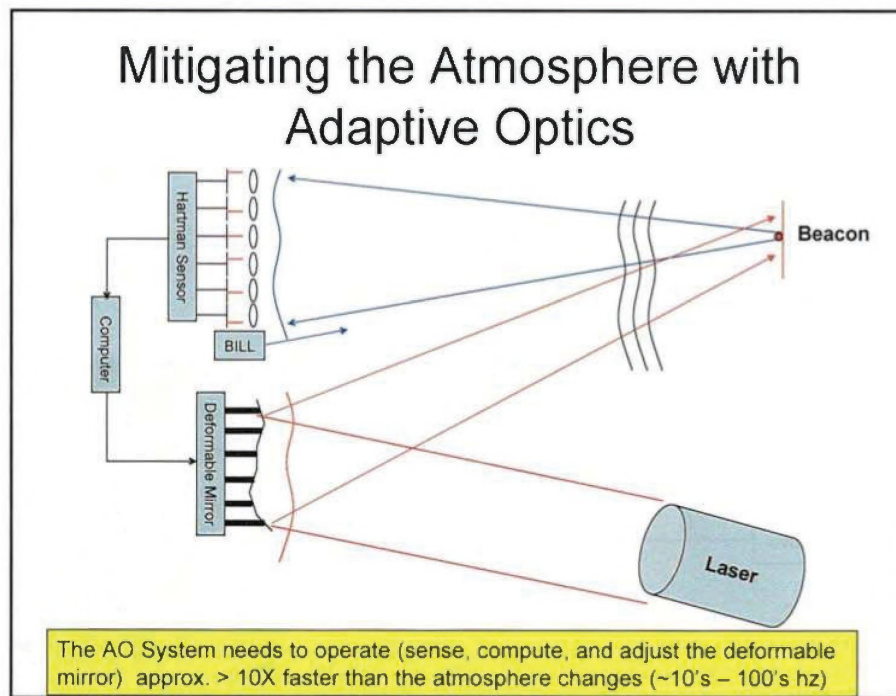
Figure 36. HEL Adaptive Optics System (courtesy of the Directed Energy Professional Society).
