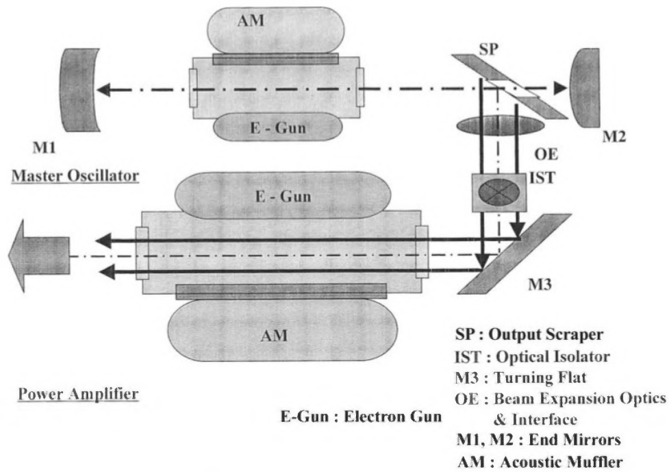
Figure 17. Schematic of MOPA [29].
