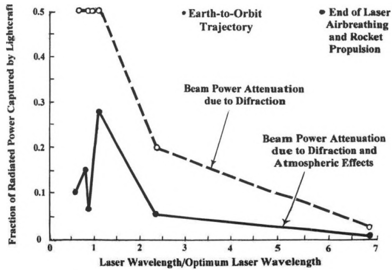
Figure 10. Attenuation Effects on Captured Laser Beam Power [26].
