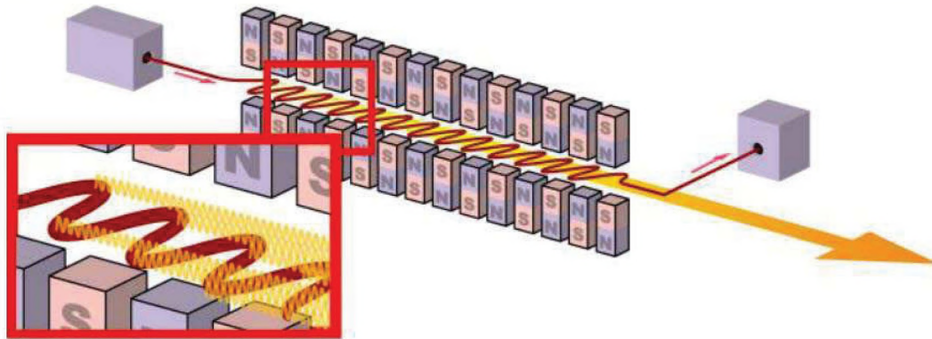
Figure 28. Free-Electron Laser (courtesy of the Naval Post-Graduate School FEL Lab).
