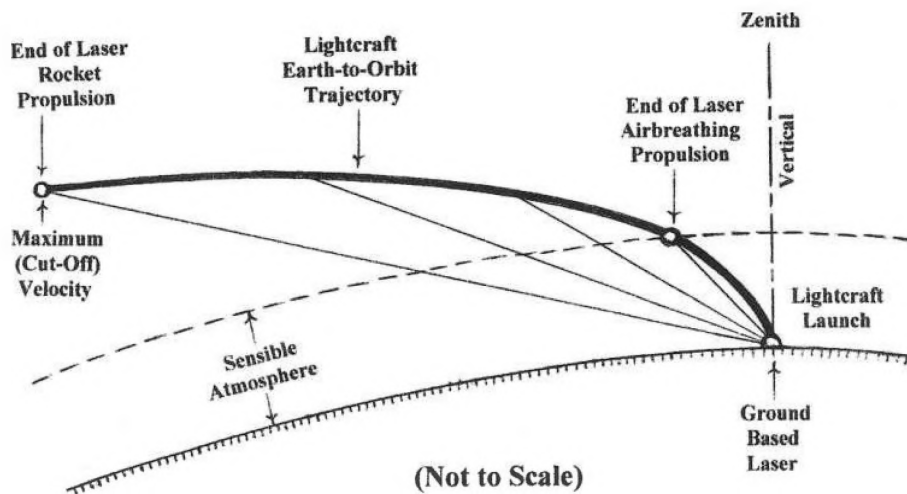
Figure 8. Lightcraft Trajectory and Associated Pointing Angles [26].
