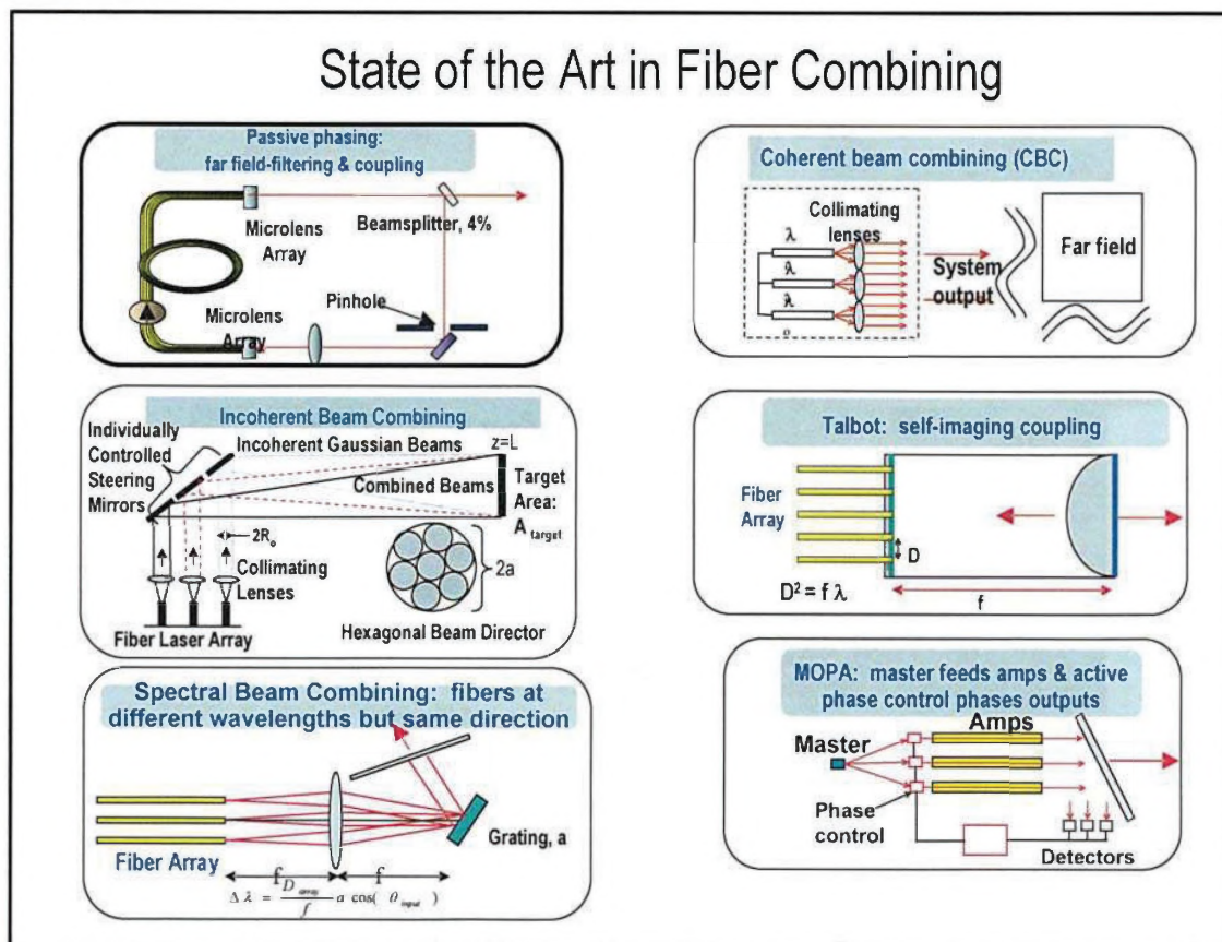
Figure 23. Fiber Laser Beam Combining Techniques (courtesy of the Directed Energy Professional Society).
