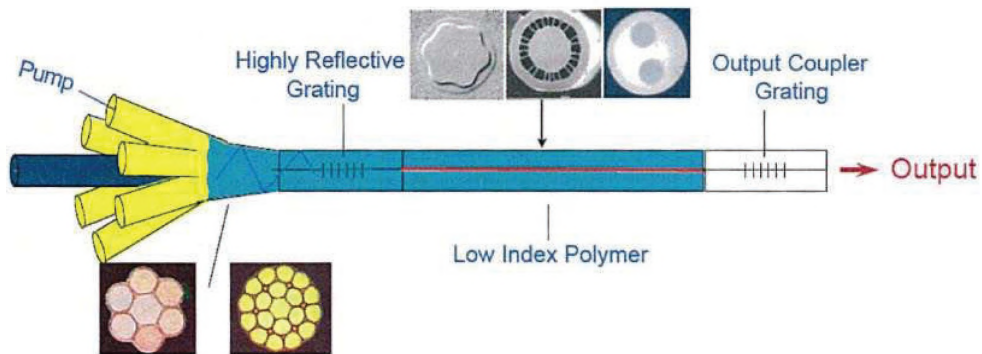
Figure 24. Pumping Fiber Lasers (courtesy of the Directed Energy Professional Society).
