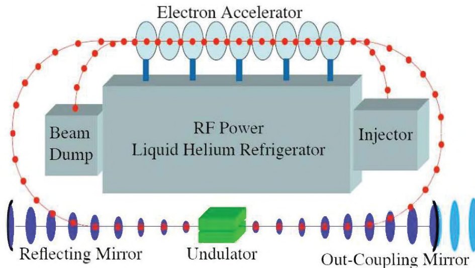
Figure 31. Recirculating-Beam FEL System (courtesy of the Naval Post-Graduate School FEL Lab).
