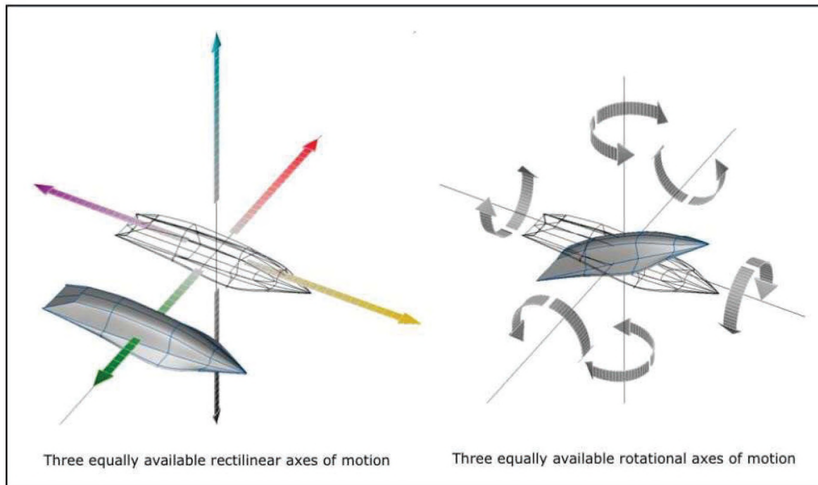
Figure 1. Six Independent Degrees of Freedom. [Graphic: A. Szames] Note: the vehicle shown is strictly hypothetical and is a combination of three 1960s science fiction vehicles: Seaview submarine, Galileo shuttle, and Amtronic car.
