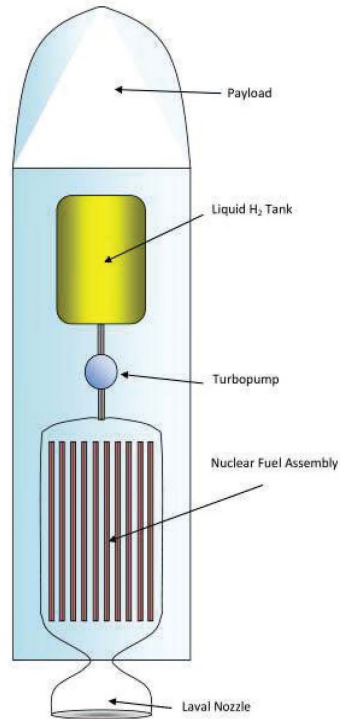
Figure 4. Nuclear Fission Rocket Design.
