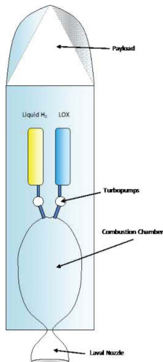
Figure 1. Liquid-Fueled Chemical Rocket.
