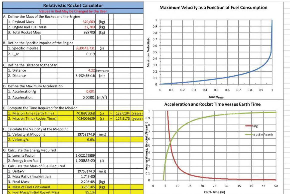
Figure 15. Spreadsheet for Sample Mission to Alpha Centauri.
