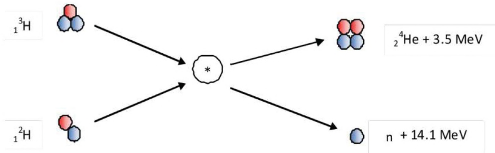
Figure 6. Nuclear Fusion of Deuterium and Tritium.
