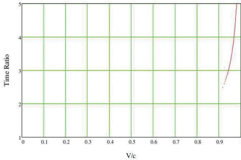
Figure 12. Time Dilation at Relativistic Velocities.
