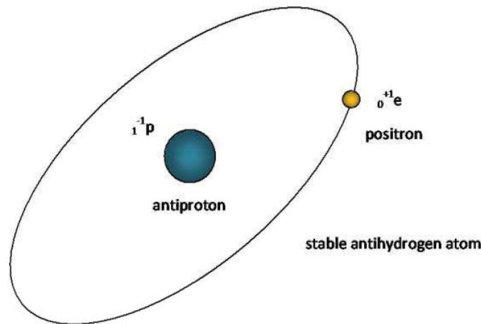
Figure 16. Antihydrogen Atom.
