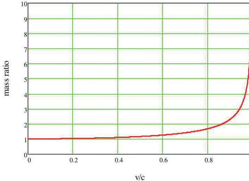
Figure 2. Mass Ratio (m/mo) Increases as Objects Approach the Speed of Light.
