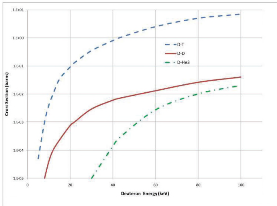
Figure 8. Fusion Ignition Energies for D-T, D-D, and D-He3.
