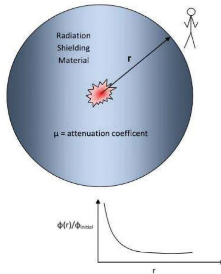
Figure 3. Spherical Radiation Shield Surrounding a Point Source.
