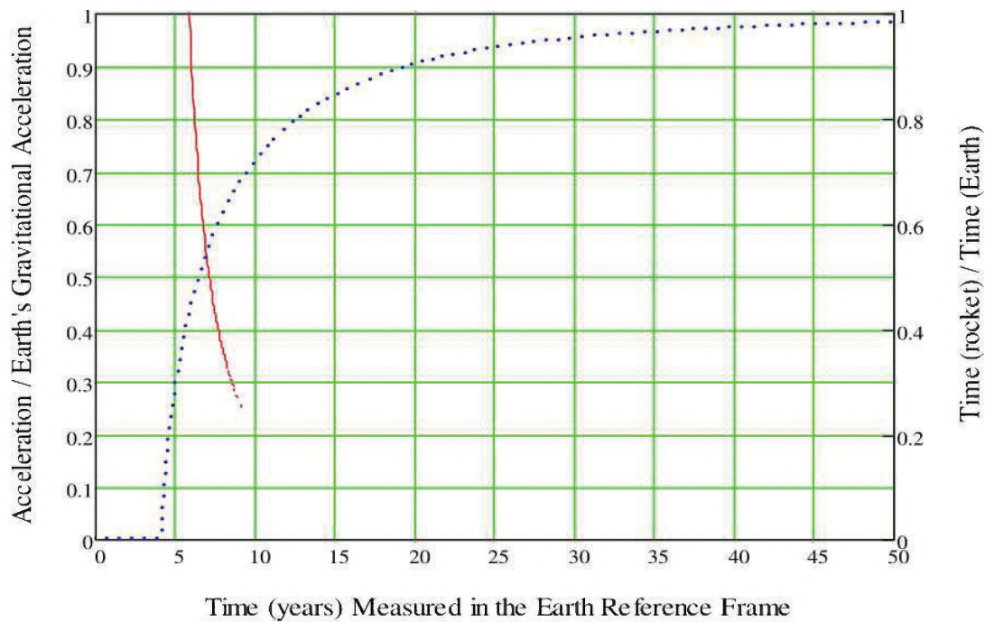
Figure 14. Acceleration and Rocket "Clock" Ratio versus Mission Time on Earth.
