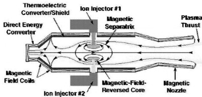
Figure 9. Colliding Beam Fusion Reactor [Cheung et al. 2004]
