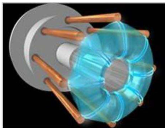
Figure 7. Dense Plasma Focus (Lawrenceville Plasma Physics)
