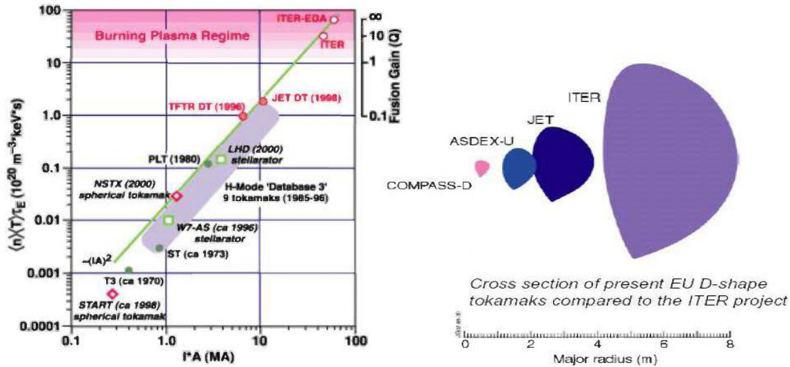
Figure 17. Progress in Tokamak Magnetic Confinement Fusion
