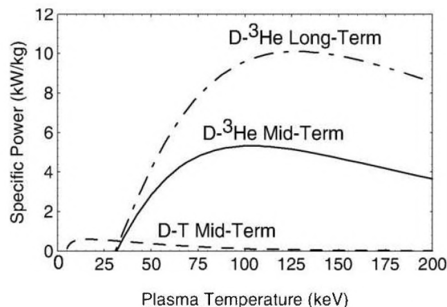
Figure 8. Specific Power as a Function of Plasma Temperature of Fusion Rocket 11
