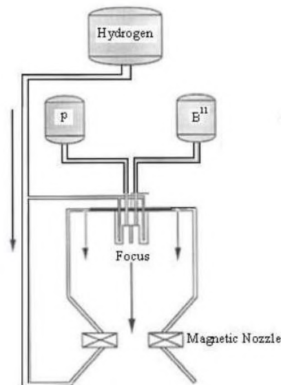
Figure 10. DPF Thruster System with Direct Conversion
