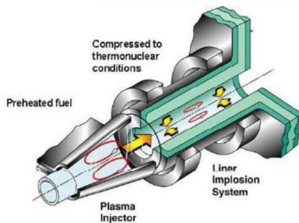
Figure 6. Magnetized Target Fusion Experiment at LANL
