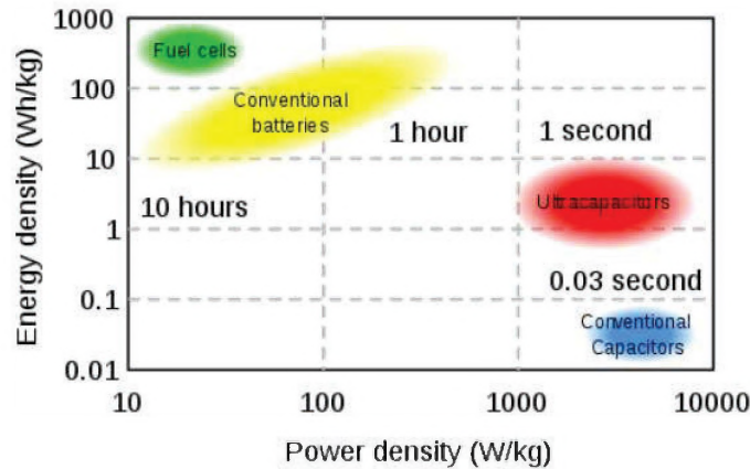
Figure 3. Ragone Plot. The graph illustrates the areas where ultracaps and batteries dominate in the power density versus energy density relationship.
