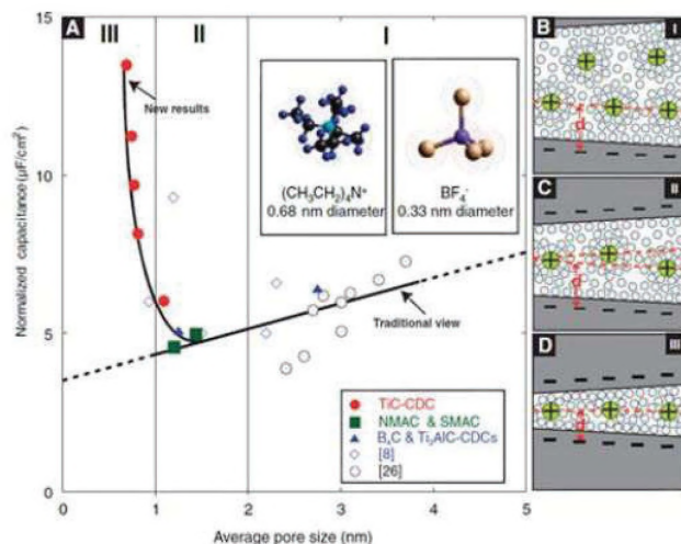
Figure 9. Relationship Between Average Pore Size and Normalized Specific Capacitance. As the average pore size decreases below 1 nm, the specific capacitance increases due to distorted electrolyte ion solvation.
