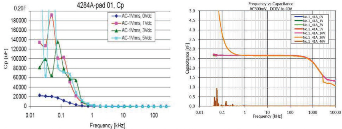
Figure 13. Preliminary MCap Test Results. These graphs demonstrate NLSC capabilities: MCap microstructure tested at different VDC (by Taiyo Yuden) (left) and single nanocell tests (right).
