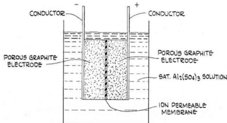
Figure 4. Electrolytic Capacitor as Designed and Patented by SOHIO.
