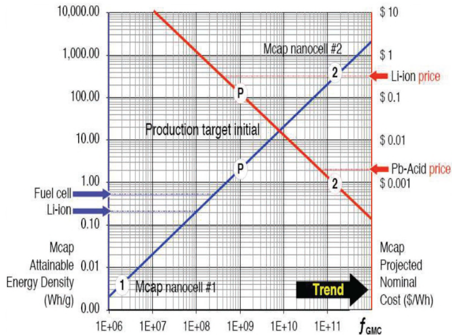
Figure 15. Specific Energy and Estimated Costs vs. f_{GMC}
