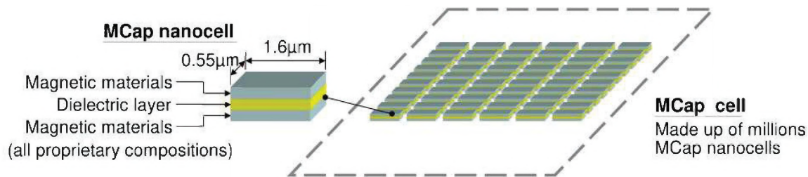
Figure 12. MCap Structure. MCap nanocell and MCap cell are fabricated using traditional semiconductor fabrication processes.
