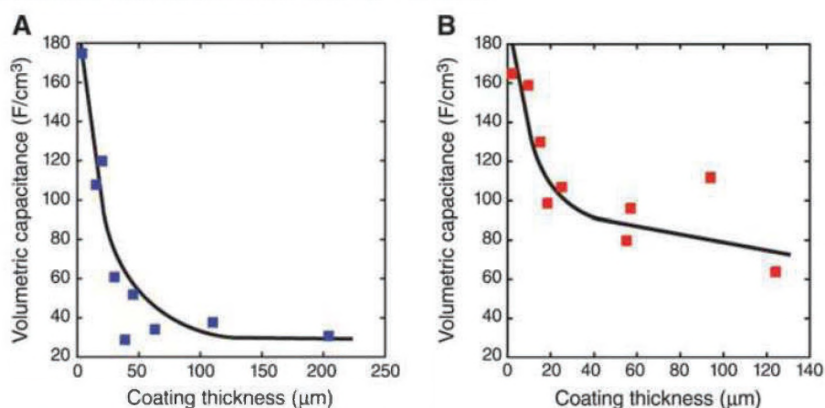
Figure 11. Volumetric Capacitance of the Films in (A) TEABF 4 and (B) H 2 SO 4 . 43
