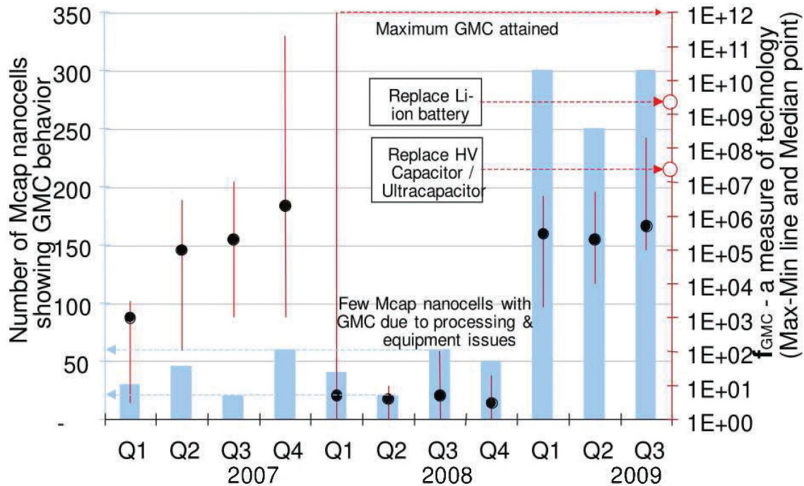
Figure 14. Summary Chart of MCap Results to Date. Right Axis: High-Low value lines in red, Median value in black dot. Left Axis: number of nanocells exhibiting GMC phenomenon in blue bar.
