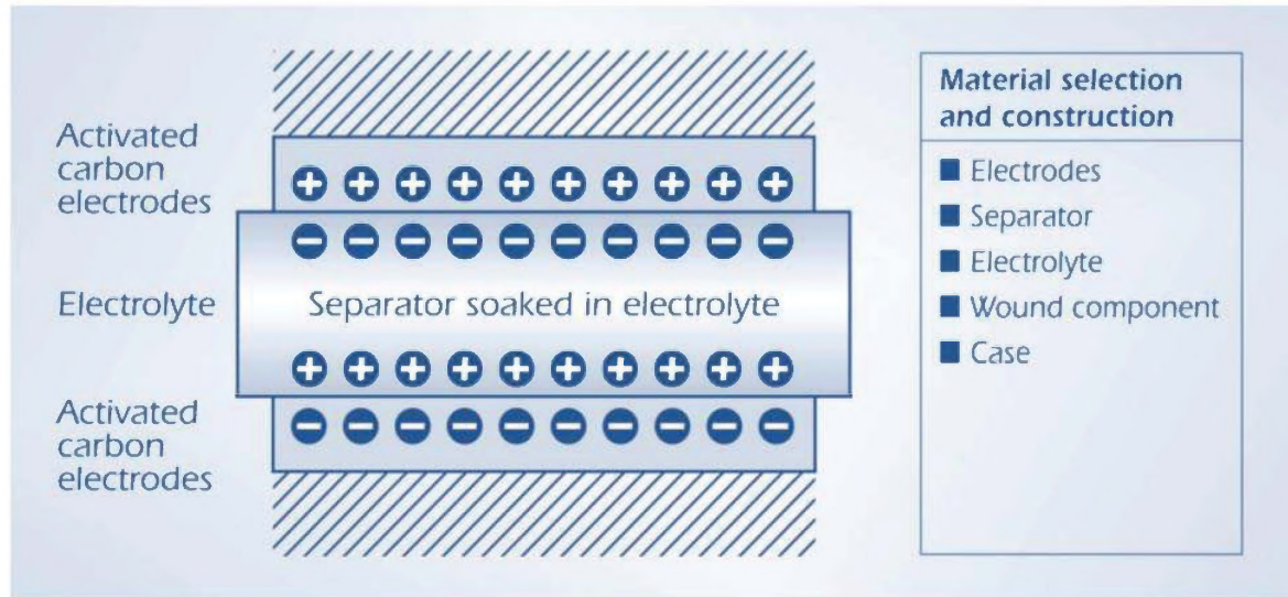
Figure 2. Operation of an Ultracapacitor. A simple ultracapacitor utilizes two similar electrodes (typically carbon) with a separator and electrolyte to create the electrochemical double layer that governs operation. 7
