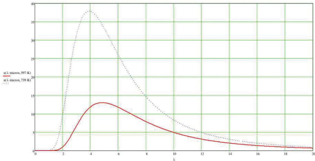
Figure 14. Infrared Energy Spectra for Mach 3 (red line) and Mach 3.5 (blue dashed line).
