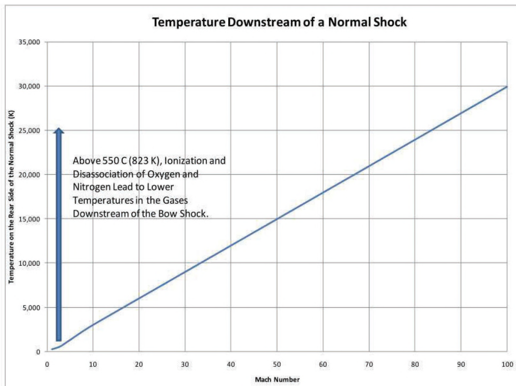
Figure 16. Peak Shock Layer Temperature for Hypersonic Objects.
