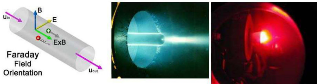
Figure 4. Electromagnetic Accelerator Field Configuration and Self-Field Electromagnetic Spacecraft Thrusters. Left: Illustration of the electric and magnetic field configuration. Center: Photograph of a MW-class pulsed magnetoplasmadynamic (MPD) thruster being tested at Princeton University. Right: Photograph of a 50-kW steady-state MPD thruster being tested at Princeton University.
