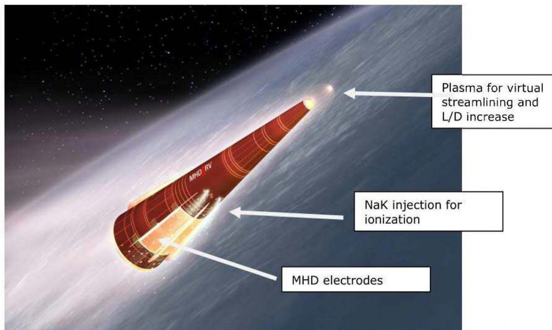
Figure 10. Reentry Vehicle With Surface-Integrated MHD Device and Plasma-Enabled Virtual Streamlining and L/D Increase.
