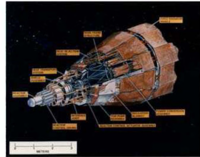
CUTAWAY VIEW OF THE SP-100 SPACE NUCLEAR POWER SYSTEM
