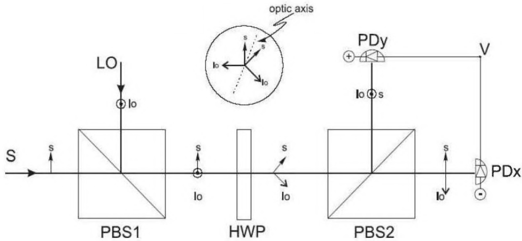
Figure 18. Detailed Schematic of Experimental BHD Apparatus. (courtesy of P. Marecki) Note that point V corresponds to point P in Figure 15.
