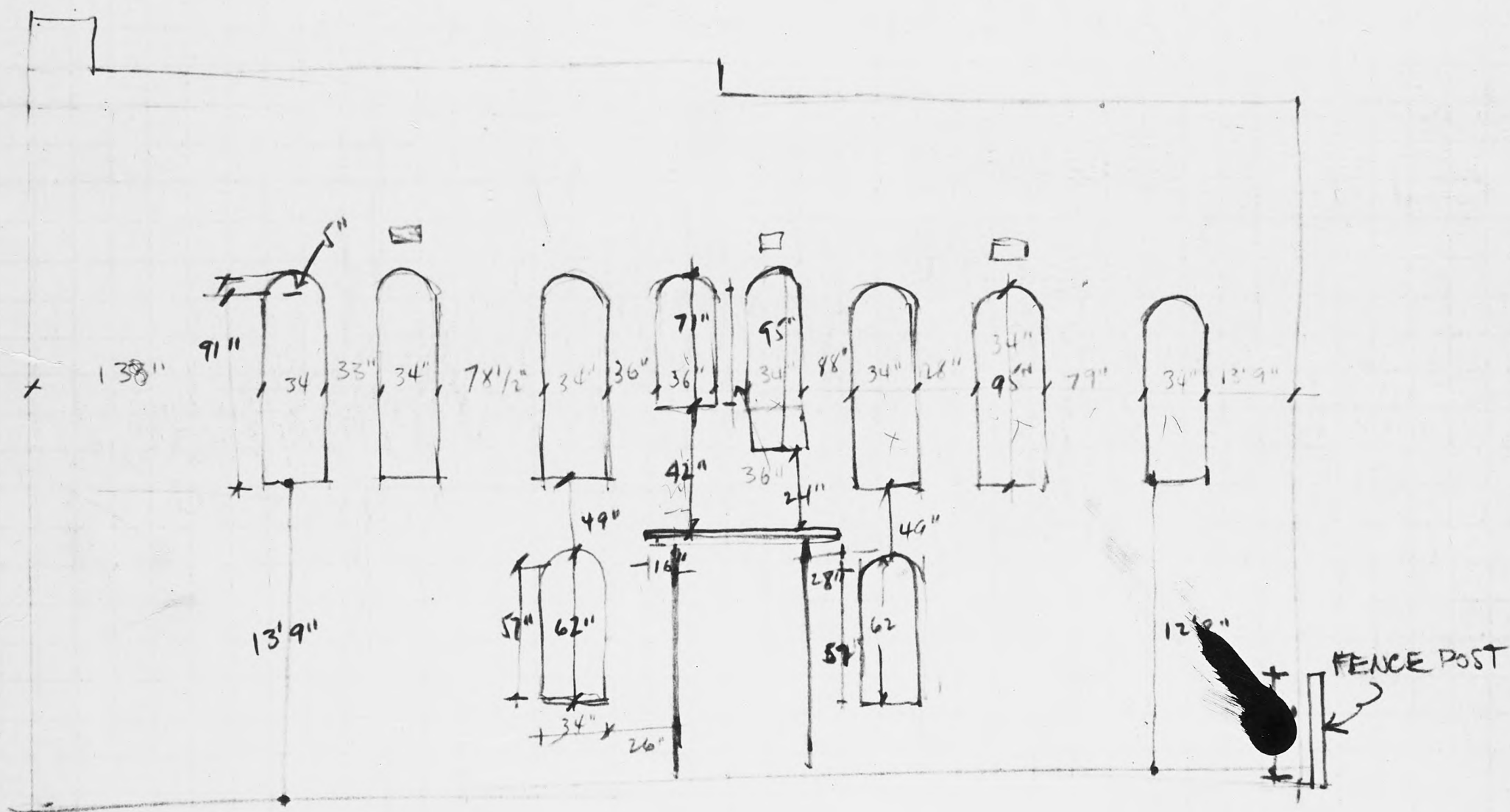
95 71 24 ELEVATION BUILDING "A" LOOKING NORTH
