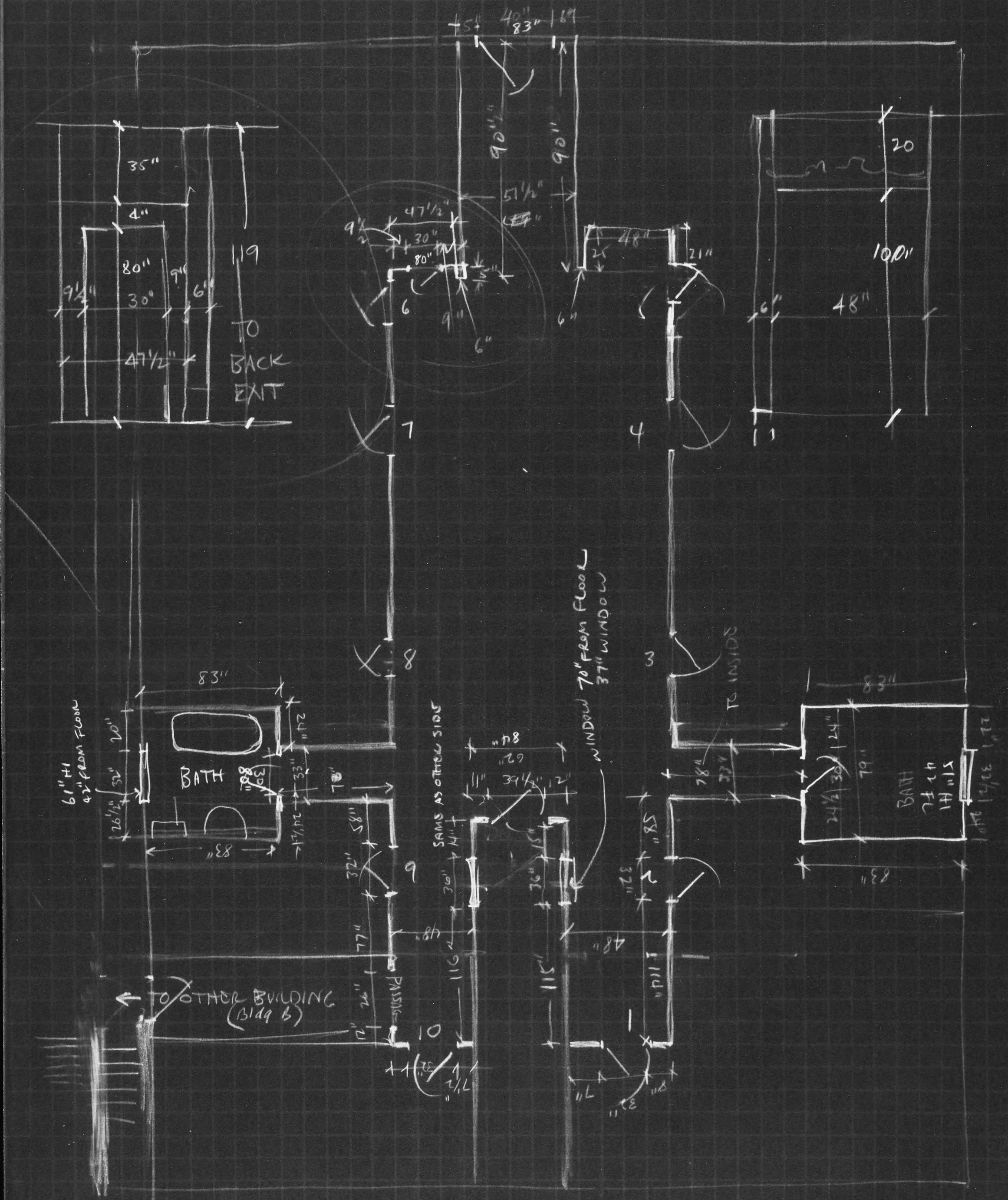
ROOMING HOUSE AT 422 1/2 S. MAIN ST., MEMPHIS FLOOR PLAN OF BLDG. A + ELEVATION BACK DOOR
