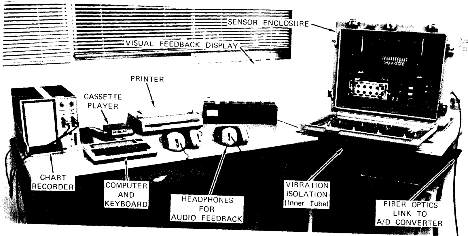
FIGURE 2 RA APPARATUS FOR PZT EXPERIMENT
