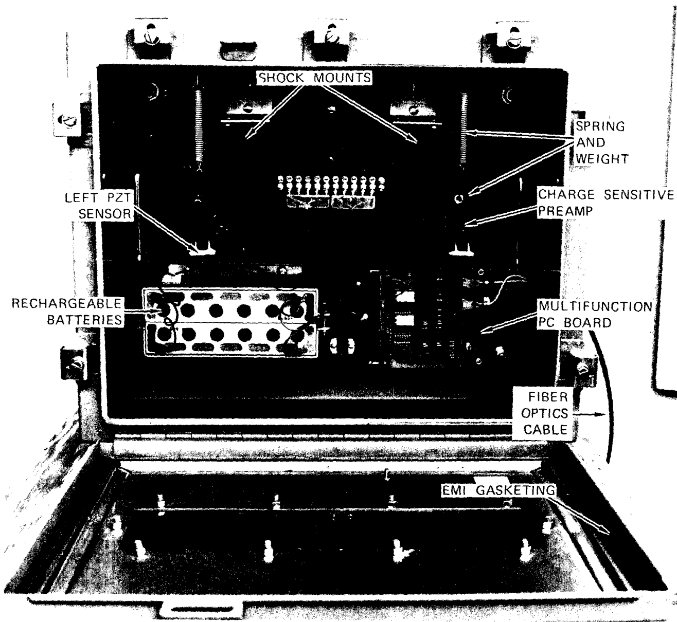
FIGURE 3 SENSOR ENCLOSURE (OPEN)
